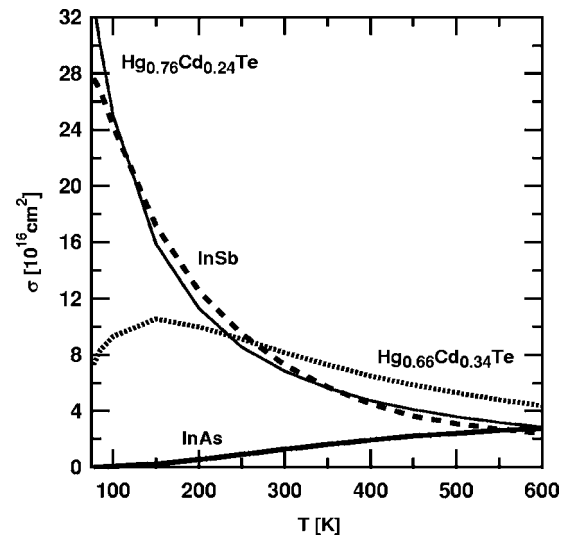
FIG. 8. Temperature-dependent free carrier absorption at 4.8\text{ }\mu\text{m} in InAs and \text{Hg}_{0.66}\text{Cd}_{0.34}\text{Te} and at 9.6\text{ }\mu\text{m} in InSb and \text{Hg}_{0.76}\text{Cd}_{0.24}\text{Te} at 300 K.
