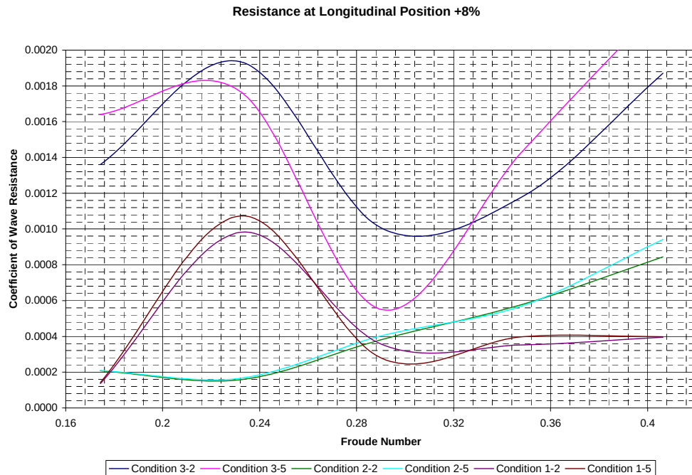
Figure 33. Wave Resistance for All Strut Combinations at a Longitudinal Position 8% of the Length of the Centerhull forward of the Transom.
