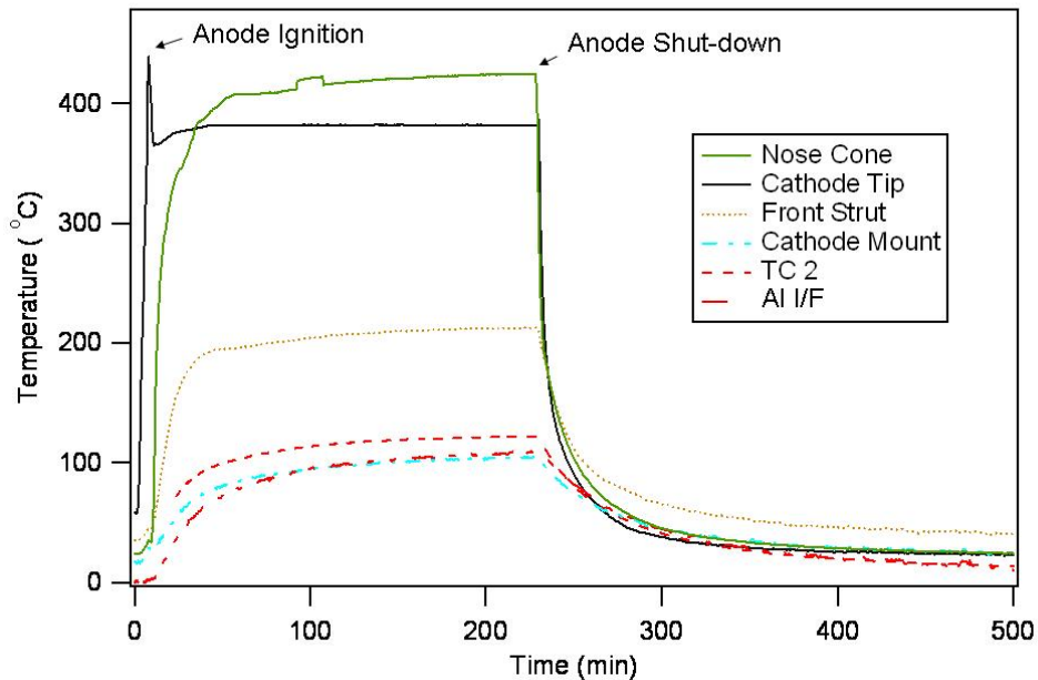
Figure 11. 200 W Thruster Temperatures versus Time for a 3.5 hour nominal burn, as seen from a 0° firing angle. Greybody emissivity is assumed.
