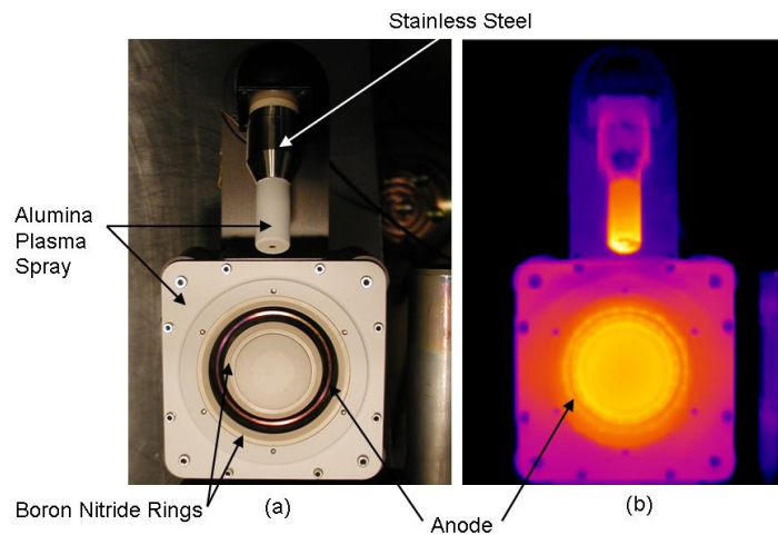
Figure 6. Busek BHT-600 Hall thruster installed on rotary stage (a) showing materials (b) IR, firing at 90^\circ
