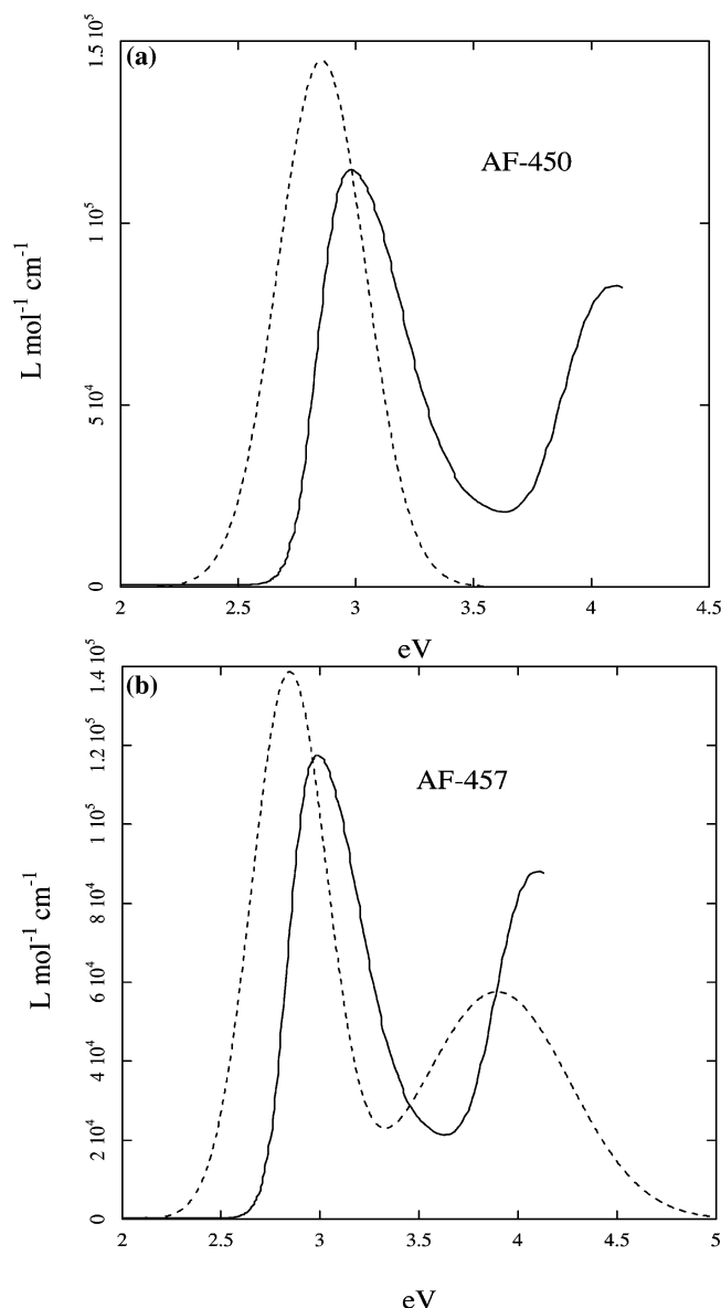
Figure 8. Experimental (in THF, solid) and computed (dash) OPA spectra of AF-450 (a, using fwhm = 0.45 eV for S_1 ) and AF-457 (b, using fwhm = 0.45 eV for S_1 and fwhm = 0.81 eV for S_2-S_n ).
