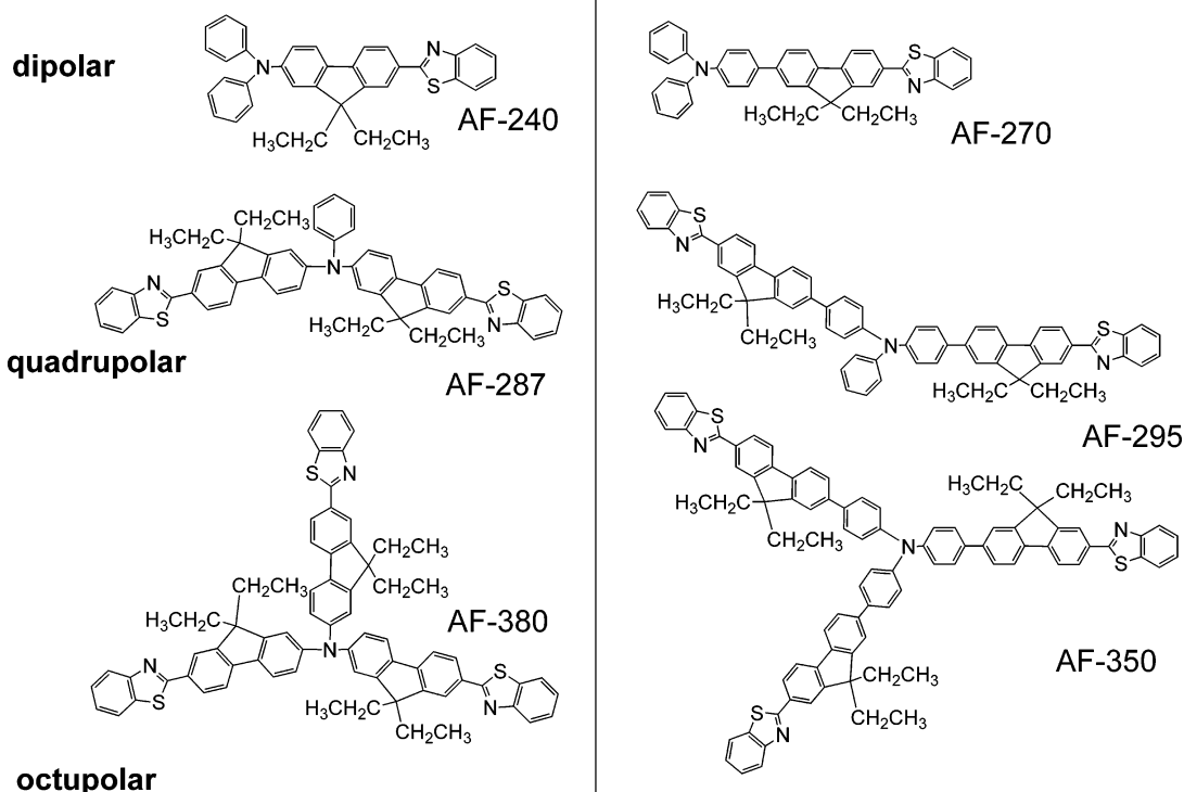
Figure 1. Structures of dipolar, quadrupolar, and octupolar chromophores.
