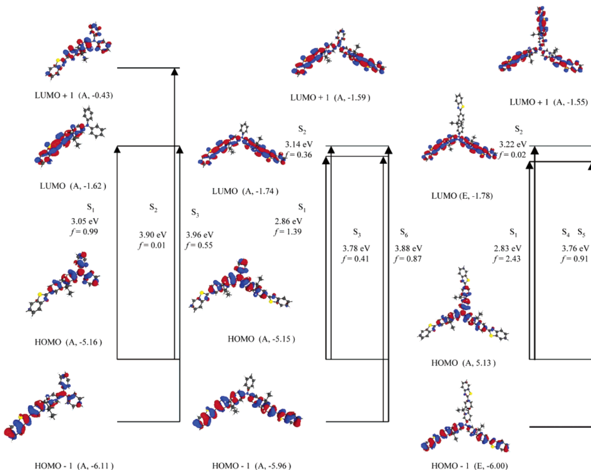
Figure 4. Molecular orbital diagrams for AF-240, AF-287, and AF-380. Solid arrows denote the major one-electron excitations.
