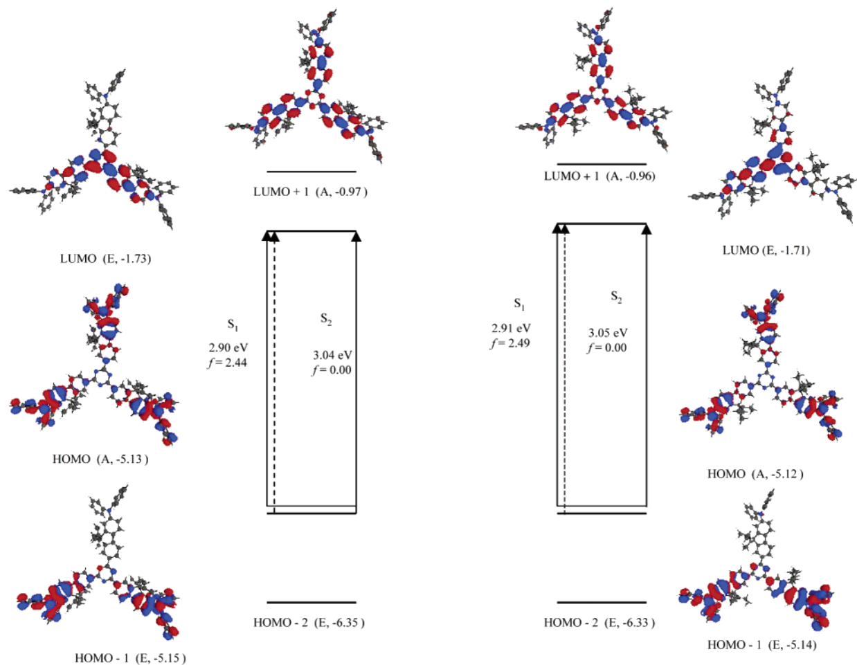
Figure 9. Molecular orbital diagrams for AF-450 and AF-457. Solid and broken arrows denote the major and minor one-electron excitations.
