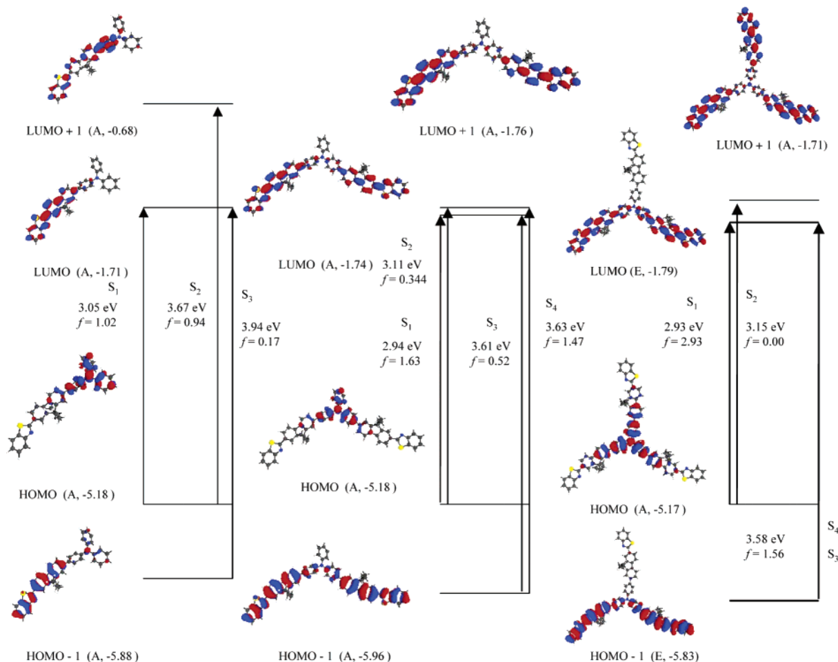
Figure 7. Molecular orbital diagrams for AF-270, AF-295, and AF-350. Solid arrows denote the major one-electron excitations.
