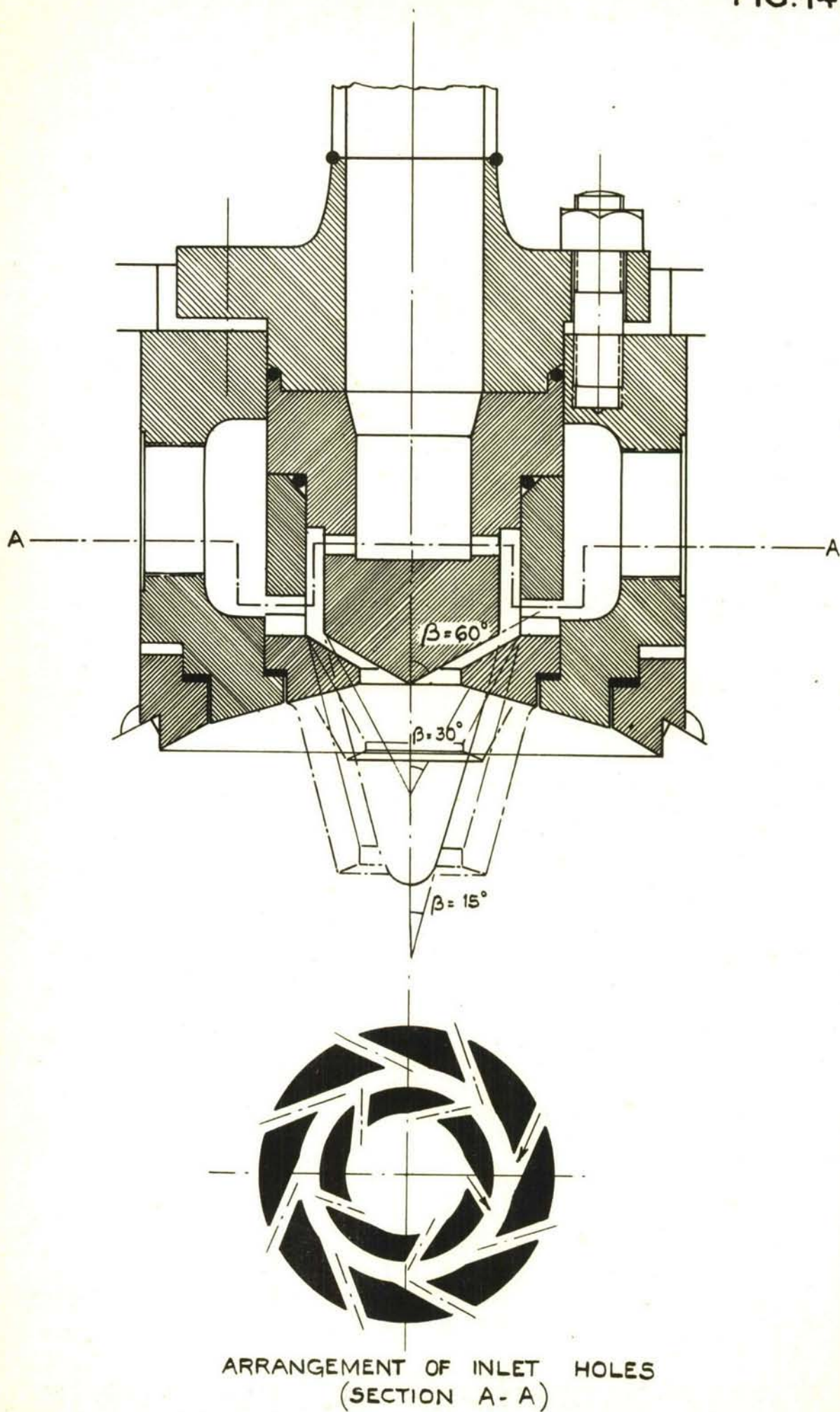
FIG. 14. JET ASSEMBLY OF NEW MIXING NOZZLE . (TYPE B) .
