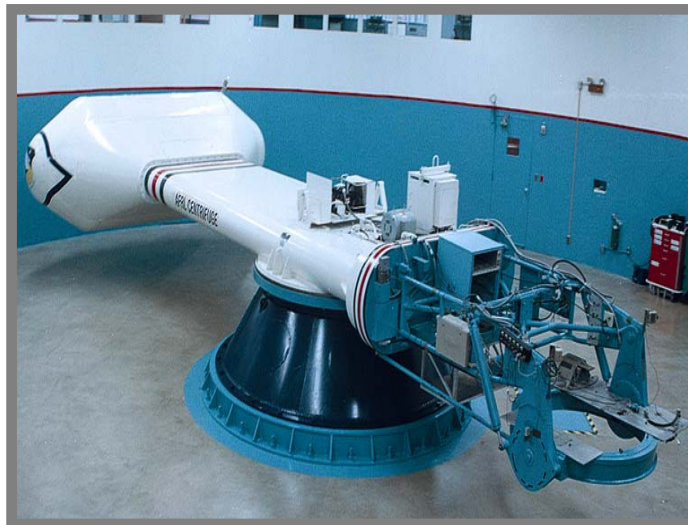
Figure 3: AFRL Centrifuge at Brooks AFB, TX
