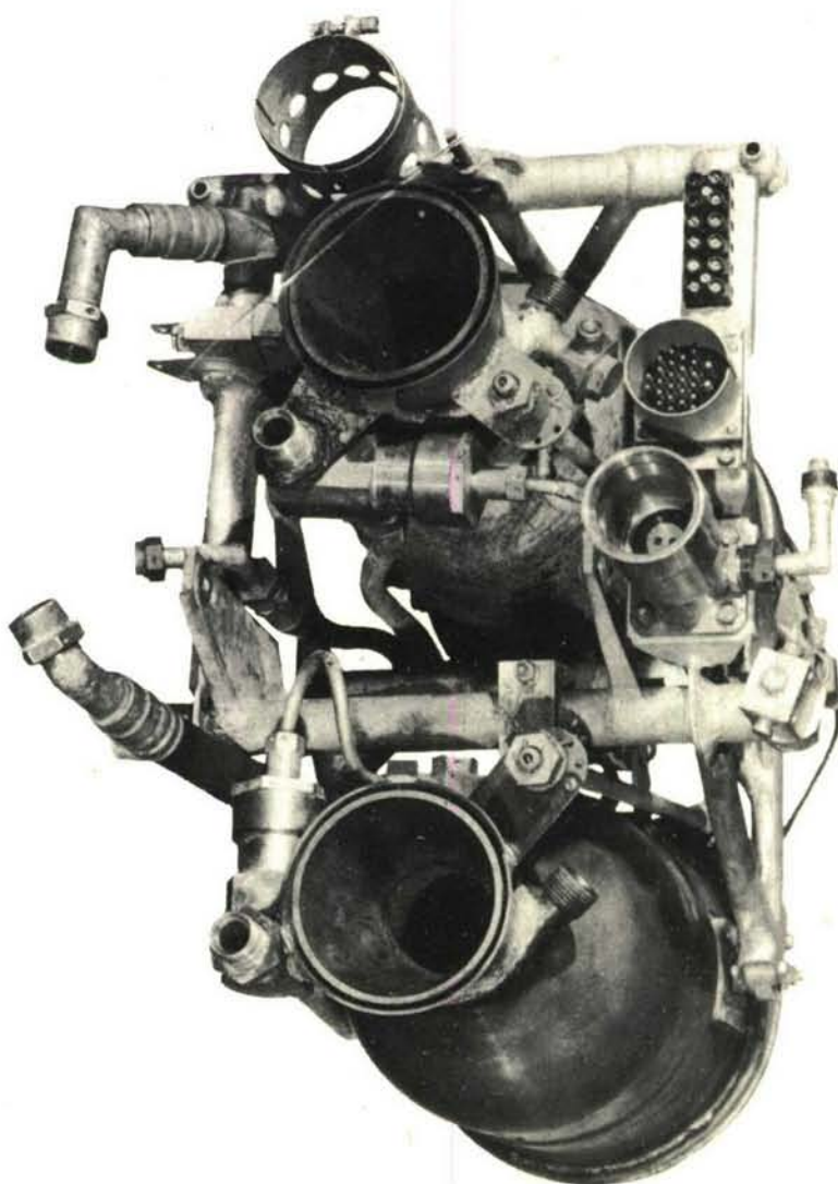
FIG.11. COMBUSTION CHAMBER UNIT
