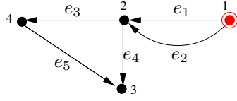
Fig. 2. A measurement Graph \mathcal{G} with node 1 as the reference node, its generalized incidence matrix \mathcal{A} , and the generalized basis incidence matrix \mathcal{A}_b constructed w.r.t. the reference node. The (block) row and (block) column indices of \mathcal{A} correspond to node and edge indices, respectively.
