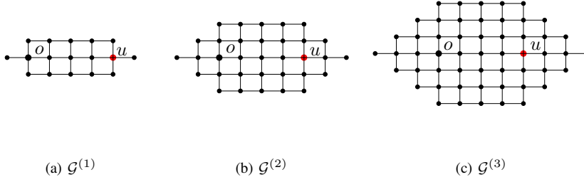
Fig. 1. A nested sequence of measurement graphs that “tend to” the 2-dimensional square lattice.
