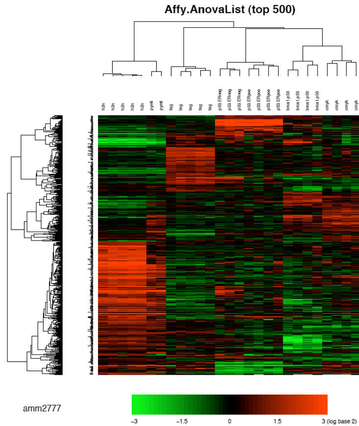
Figure 4. 500 top genes (p value rank) to generate two-way clustering heatmap. The hierarchical clustering analysis shows clear model-specific signatures, which are robustly preserved across the gene selections described above.
