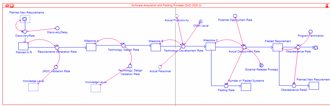
Figure 14. System Dynamics Model Representation of DoD Acquisition System
