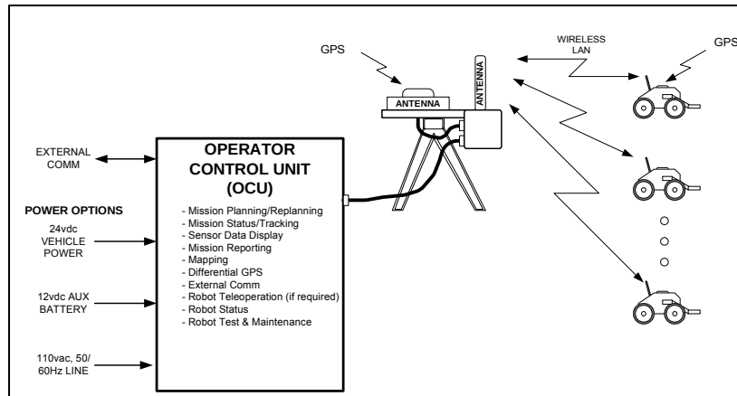
Figure 8. The GDRS BUGS block diagram.
