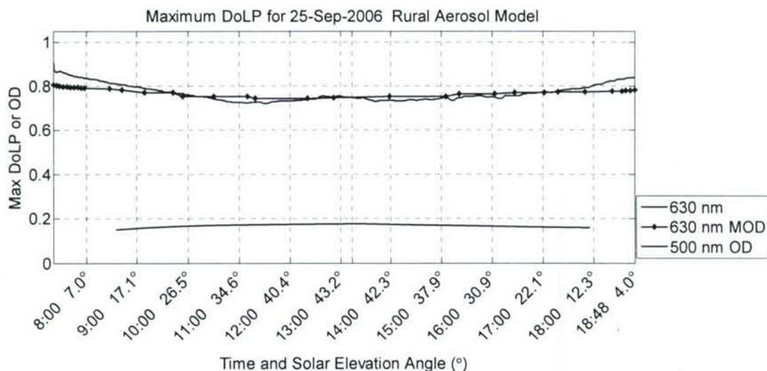
Figure 30. Low-aerosol max DoLP with Rural single-scatter model 630 nm.
