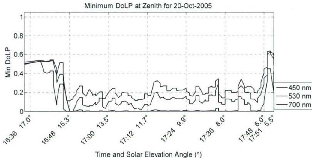
Figure 12. Minimum DoLP at zenith using the telephoto lens on October 20, 2005.
