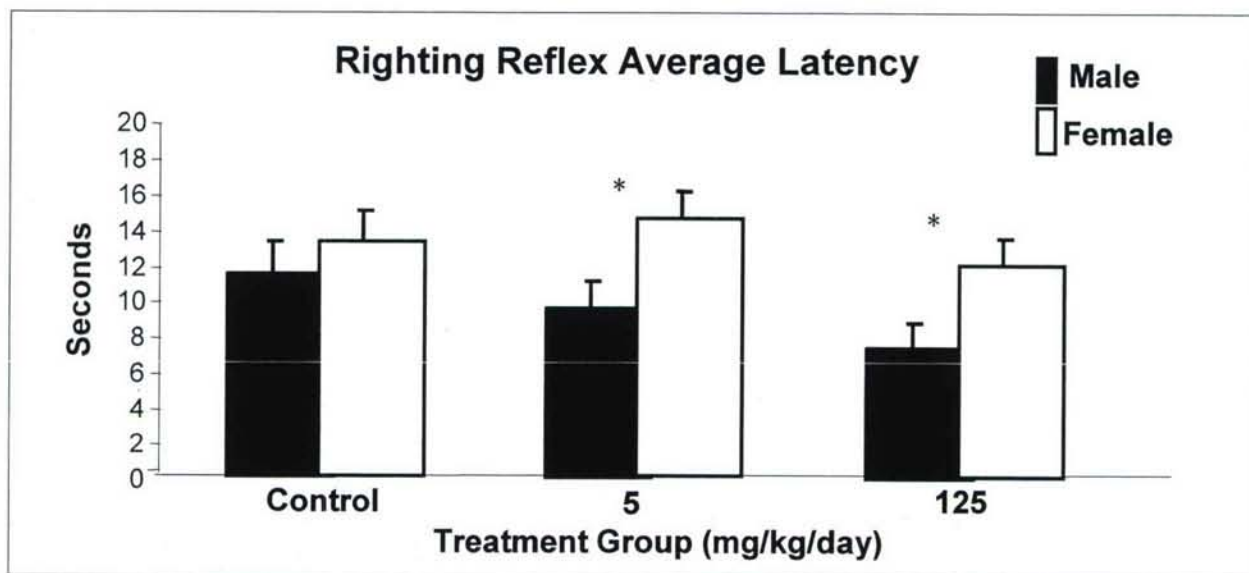
Figure 1. Righting Reflex Average Latency for Pups.
