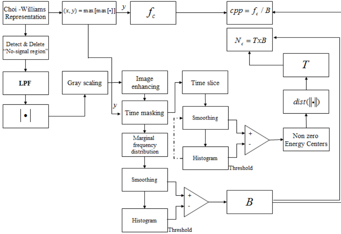
Figure 64. Parameter Extraction Block Diagram for polyphase coded LPI radar modulations using CWD images.
