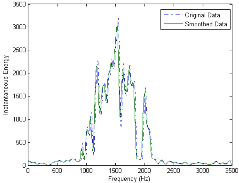
Figure 32. Output of Moving Average Filter with a Window Length of 10.
