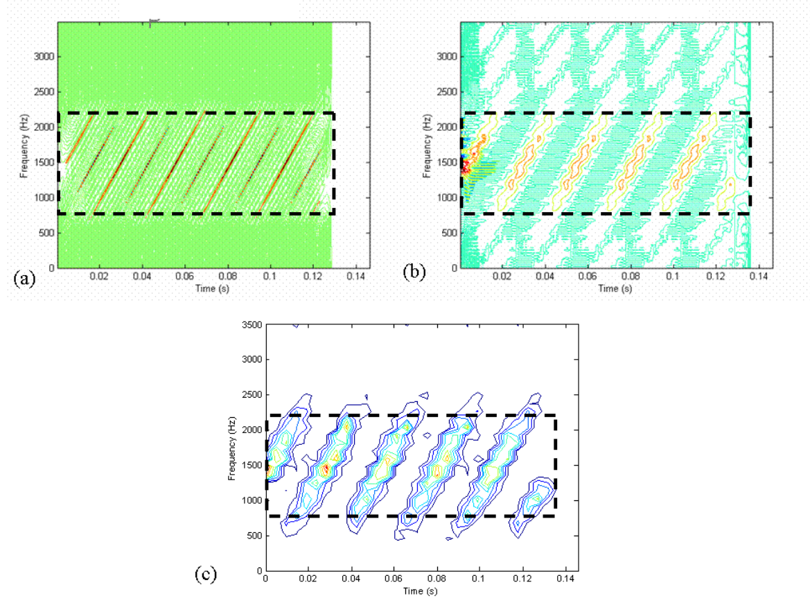
Figure 19. The Frequency Bands of Interests (a) PWVD (b) CWD (c) QMFB.
