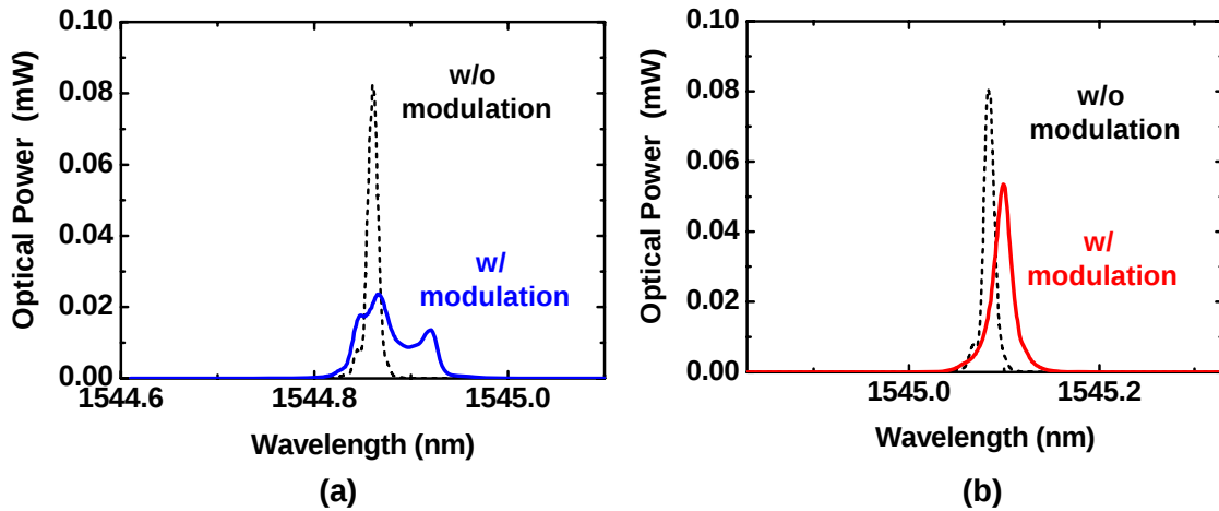
Figure 5-18. Measured optical spectra of the two-section DFB lasers under direct modulation with 10-Gb/s NRZ data: (a) I_1 = 90 mA, I_2 = 0 mA; (b) I_1 = 90 mA, I_2 = 30 mA. The optical power is measured in linear scale. The optical spectra without data modulation are depicted as dotted lines.
