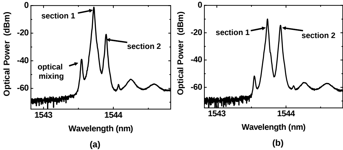
Figure 5-9. Optical spectra measure at the facet facing at (a) section 1 and (b) section 2. Bias current is I_1 = 30 mA and I_2 = 21 mA.
