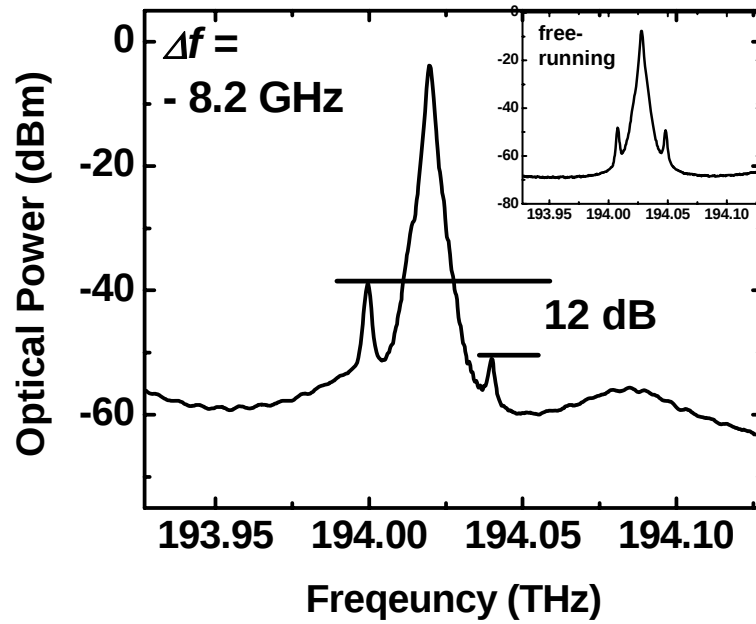
Figure 3-12. Measured optical spectrum of RF-modulated injection-locked laser ( f_m = 20 \text{ GHz} ).
