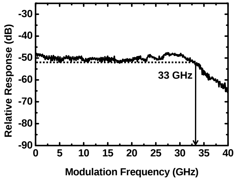
Figure 2-12. Experimental results showing broadband response. The injection ratio R is set at 18 dB.
