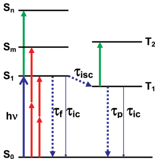
Scheme 1. Energy Level Diagram and Summary of Spectroscopic Measurements a
