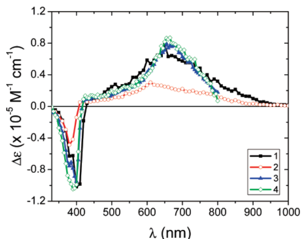
Figure 4. T_1-T_n absorption spectra observed after nanosecond-pulsed 355 nm excitation of 1 (5.9 \mu M), 2 (2.5 \mu M), 3 (3.0 \mu M), and 4 (1.7 \mu M) in deoxygenated benzene. Samples were deoxygenated by the freeze–pump–thaw method. Molar extinction coefficients were obtained by using the method of relative actinometry.
