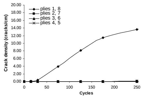
Figure 5: Damage in IM7/5250-4 [0/90] 2s (-196 °C to 177 °C thermal cycling)
