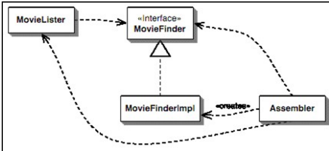
Figure 133. An illustration of IoC from Fowler, Martin. (2007). IoC. Retrieved September 5, 2007 from http://martinfowler.com/articles/injection.html . The diagram is showing the IoC framework or assembler creating a runtime concrete class dependency for a MovieLister based on an XML descriptor. In the XML descriptor, the persistence type (CSV, SQL, etc.) is tied to a specific concrete class, i.e., SQLMovieFinderImpl.java or CSVMovieFinderImpl.java making the MovieLister code much more reusable and modular.
