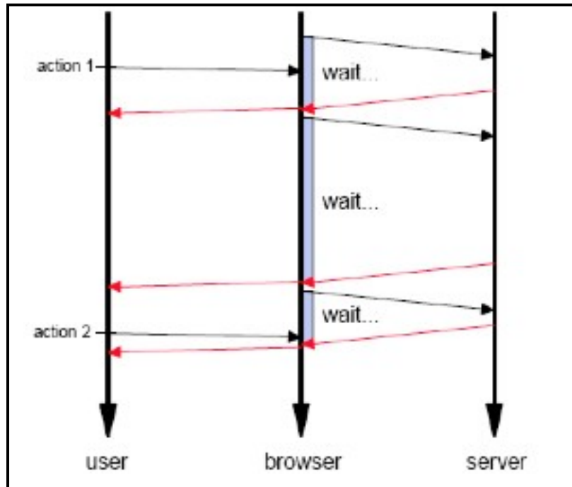
Figure 23. A diagram showing Ajax Asynchronous Polling (Smart Polling) from [24]. Note that in this new model, the polling wait times are vary. In the asynchronous-mode polling reacts much better to network lag and server-load, making it a better solution if massive scalability is a concern.
