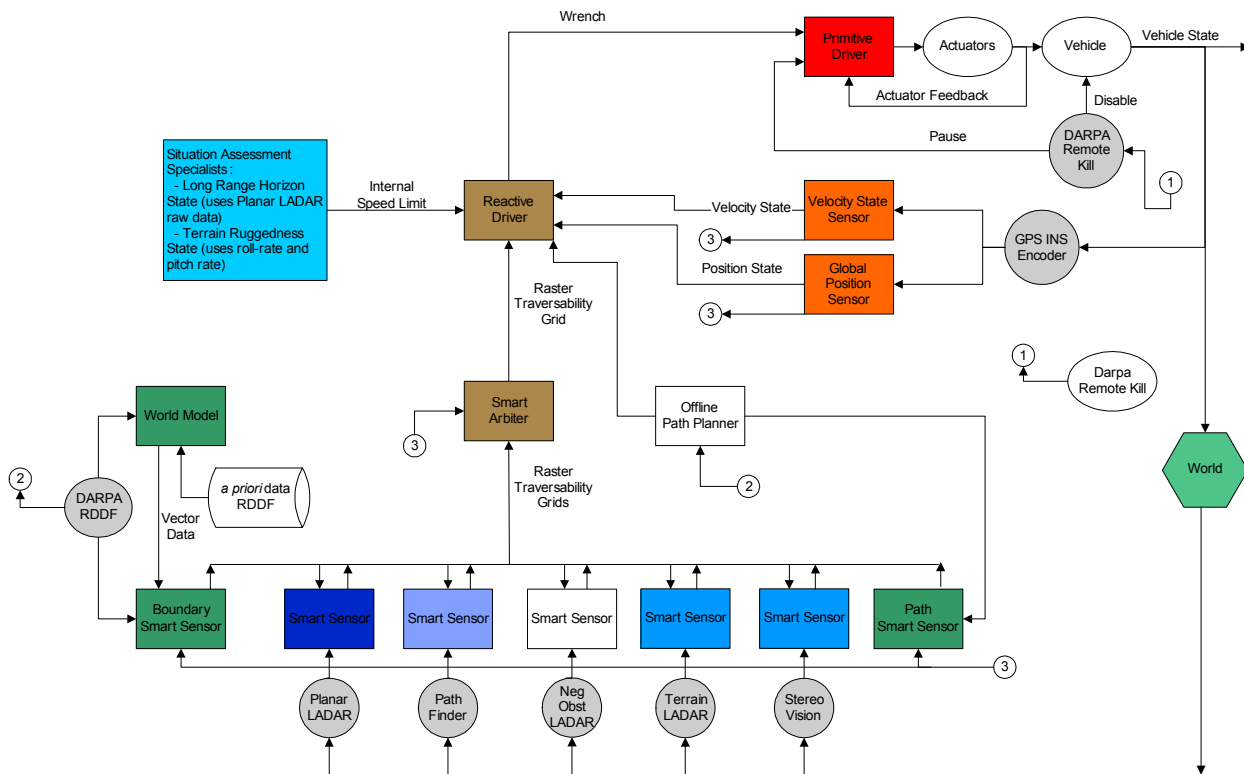
Figure 1-3. As-built NAVIGATOR Component Block Diagram used in 2005 DARPA Grand Challenge.
