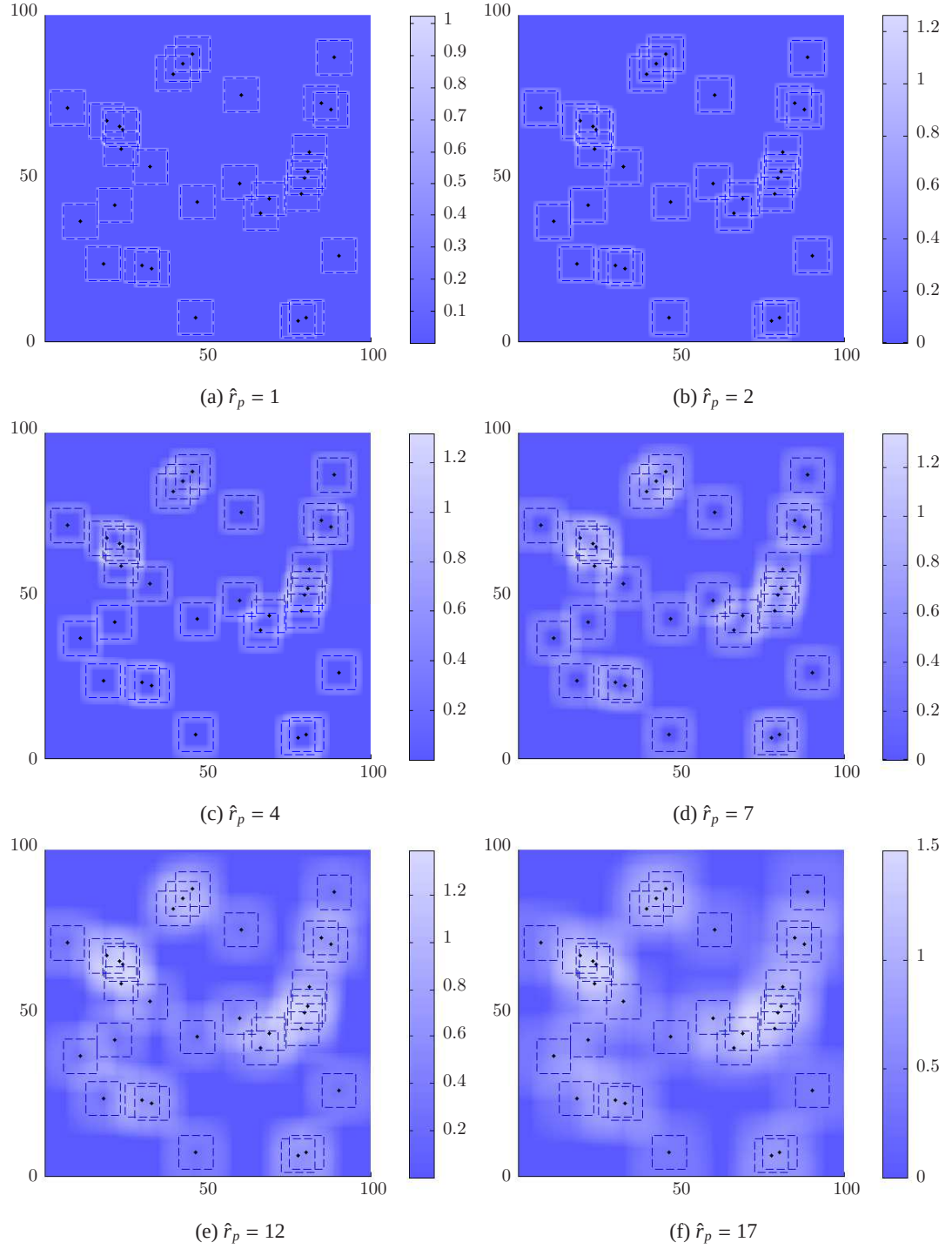
Figure 5.3: Information maps computed using discrete, binary sensors and an uniform prior with varying radius \hat{r}_p as detailed in Table 5.1.
