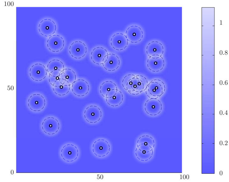
Figure 6.6: Information map using the improved models. White dots outlined in black represent nodes, and dotted circles represent their detection region. Background color of the plot represents the amount of information.
