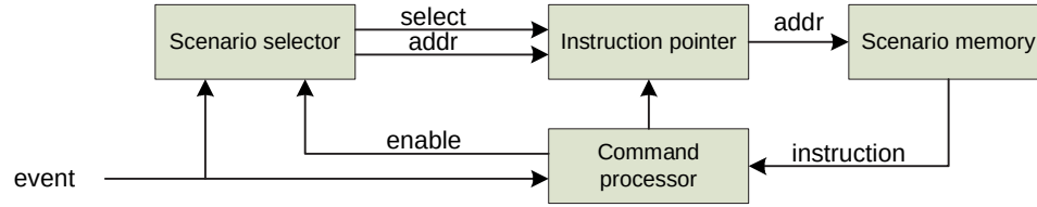
Figure 4.4: Block diagram of scenario scheduler inside PM.
