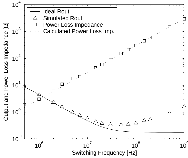
Figure 21: Simulated output impedance with parasitics
