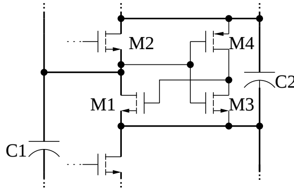
Figure 12: Latch-based gate drive
