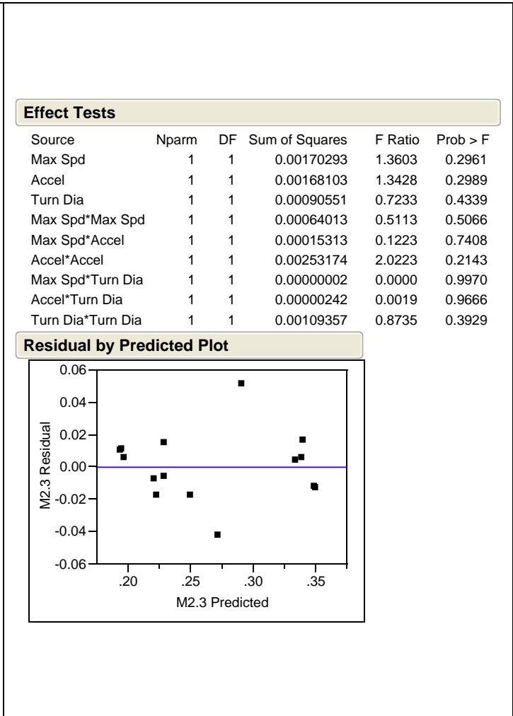
Figure B11. Summary of Initial Model Fit For M2.3 (continued)
