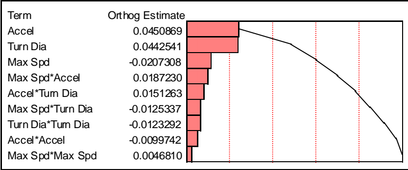
Figure B3. Pareto Plot For M2.1 Initial Fit
