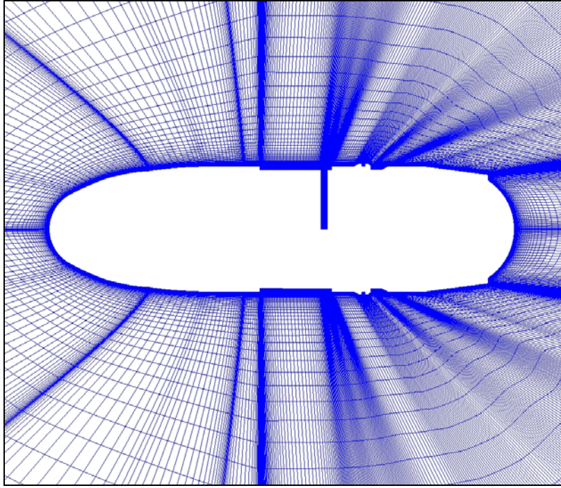
Figure 4. Computation mesh, axisymmetric view showing internal cavity.
