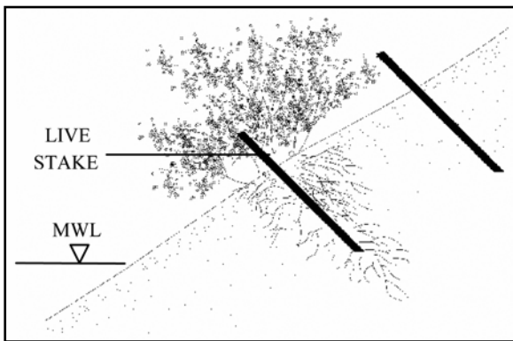
Figure 6. Development of a live stake installation
