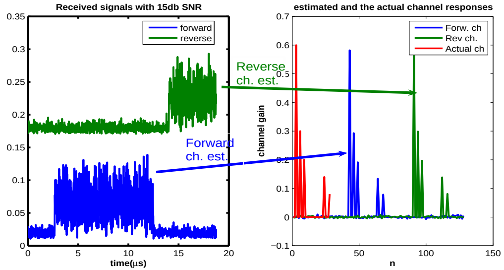
Figure 6.3: Simulated waveforms during forward and reverse transmissions (Left), Estimated reverse, forward and the actual channels. (Right)
