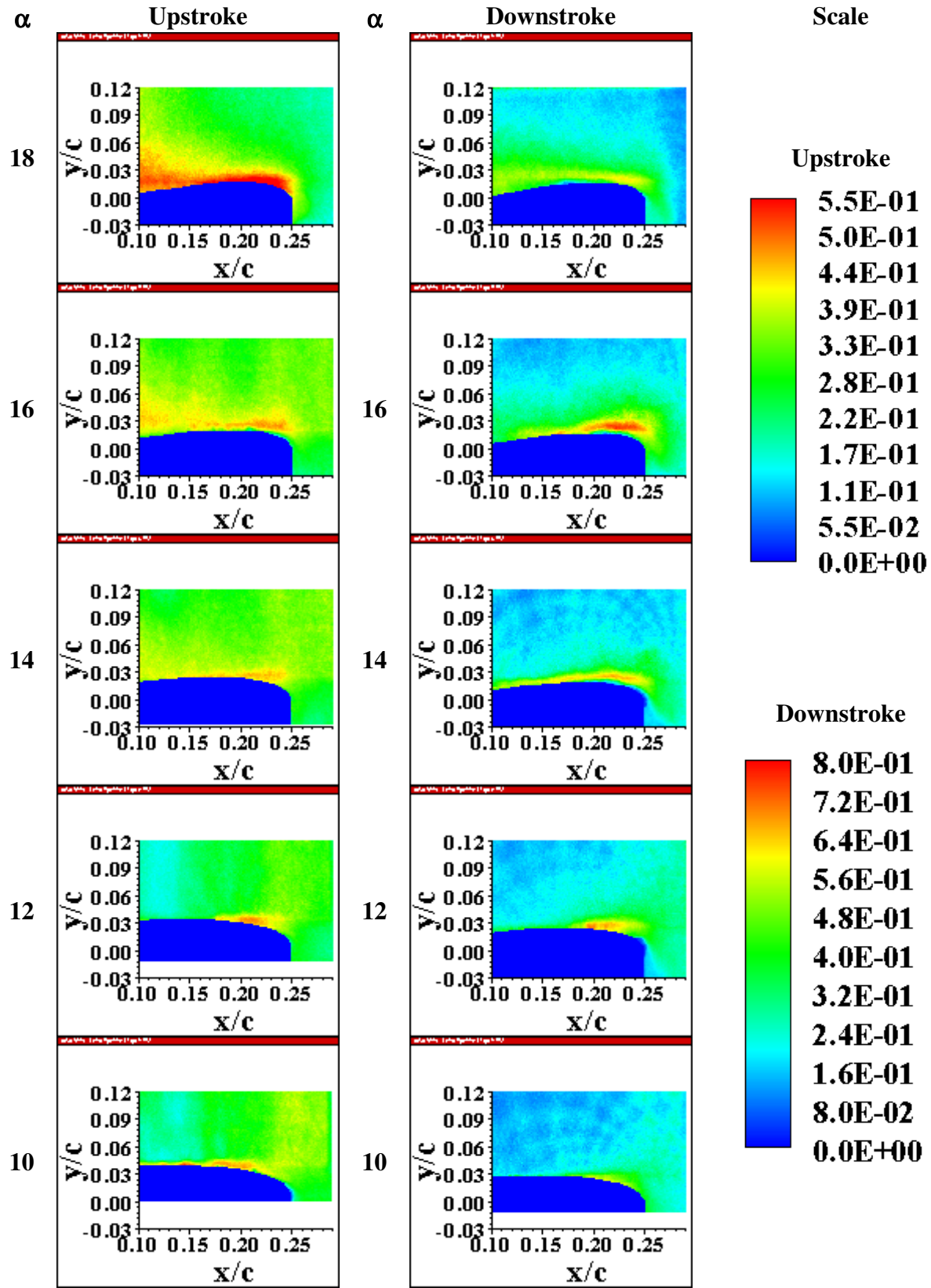
Figure 6.9 u/c , Case 2 ( M = 0.28 , k = 0.1 , \Delta\alpha = 10 deg)
