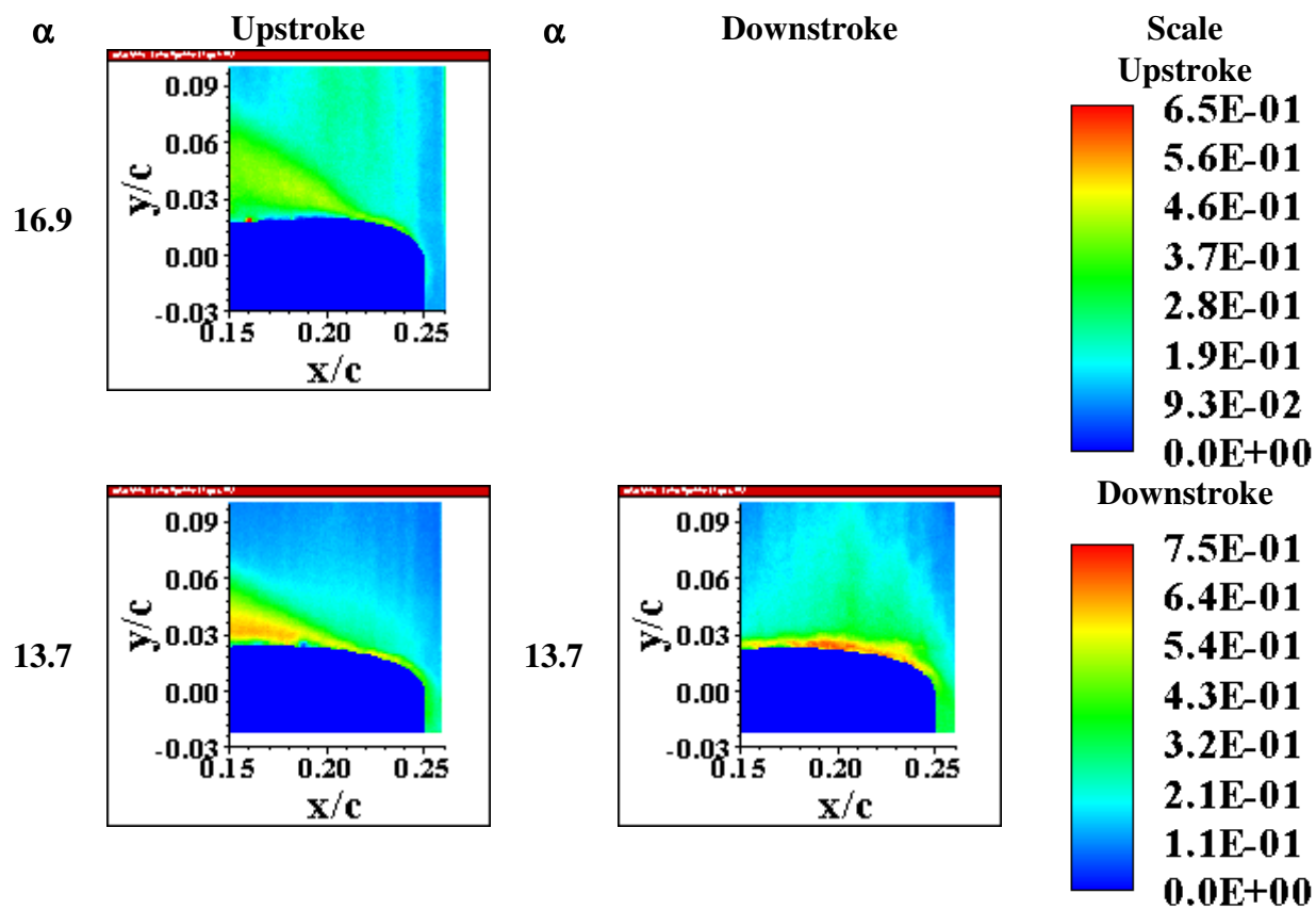
Figure 6.18 \sigma_u , Case 4 ( M = 0.2 , k = 0.18 , \Delta\alpha = 5 deg)
