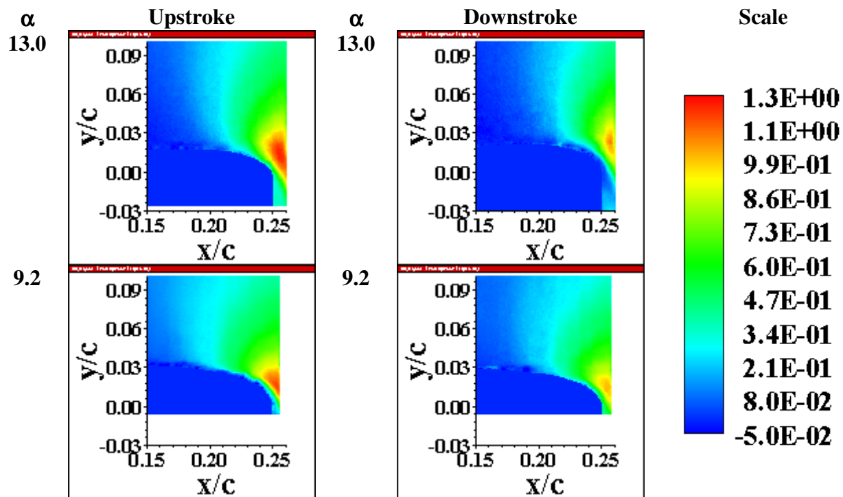
Figure 6.12 V/U_\infty , Case 3 ( M = 0.2 , k = 0.18 , \Delta\alpha = 5^\circ )
