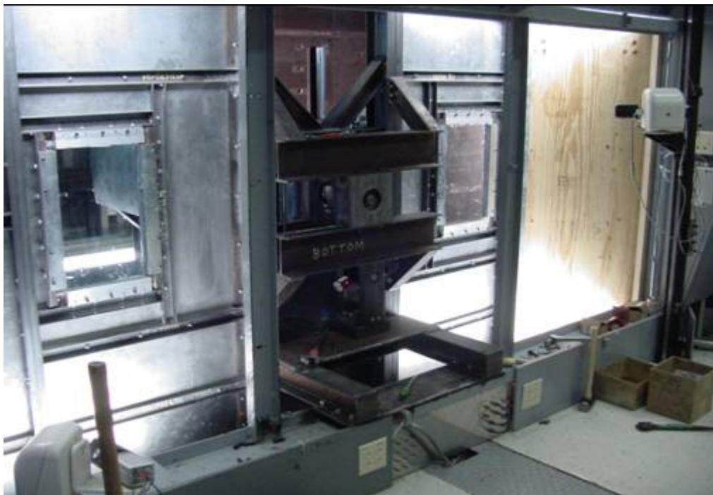
Figure 4.57 Wing vibration and load support structures in-place
