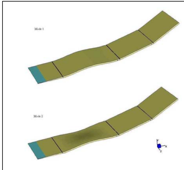
Figure 3-8: Vibration frequencies of intake at a uniform temperature of 300K and 30 km altitude. Displacement scale = 1.5%
