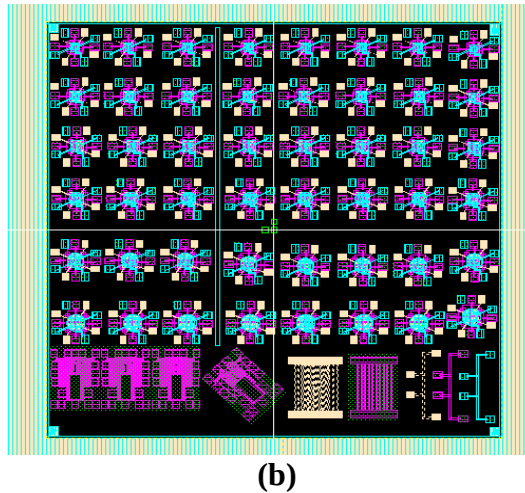
Figure 4.6: (a) FLEMS sensor layout (b) View of test die containing devices of various sizes and test structures (for measurement of stress, strain gradient, resistivity, and Young's Modulus).
