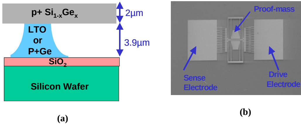
Figure 3.4: (a) Schematic cross-section of cantilever beam used to determine the strain gradient in structural poly- \text{Si}_{1-x}\text{Ge}_x films. (b) SEM micrograph of fabricated comb-drive test structure.
