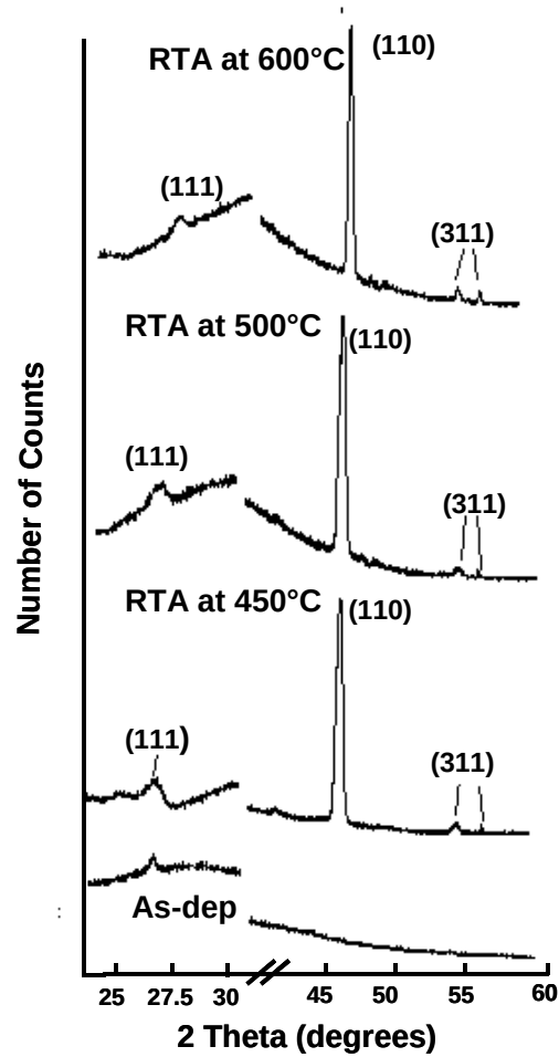
Figure 3.16: XRD results of as-deposited as well as annealed p+ \text{Si}_{1-x}\text{Ge}_x films at different RTA (Rapid Thermal Annealing) temperatures. RTA was performed in a \text{N}_2 ambient.
