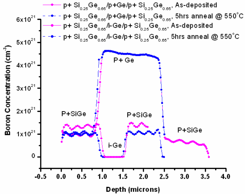
Figure 3.18: Boron concentration verse depth using SIMS analysis (accuracy with 2-3%) For the two tri-layers: p+Si 0.25 Ge 0.65 /p+Ge/ p+ Si 0.25 Ge 0.65 and p+Si 0.25 Ge 0.65 /i-Ge/ p+ Si 0.25 Ge 0.65 , Boron concentration is compared for As-deposited films and annealed films. Note that the slight shift observed is accounted through the 2.5% accuracy of SIMS analysis.
