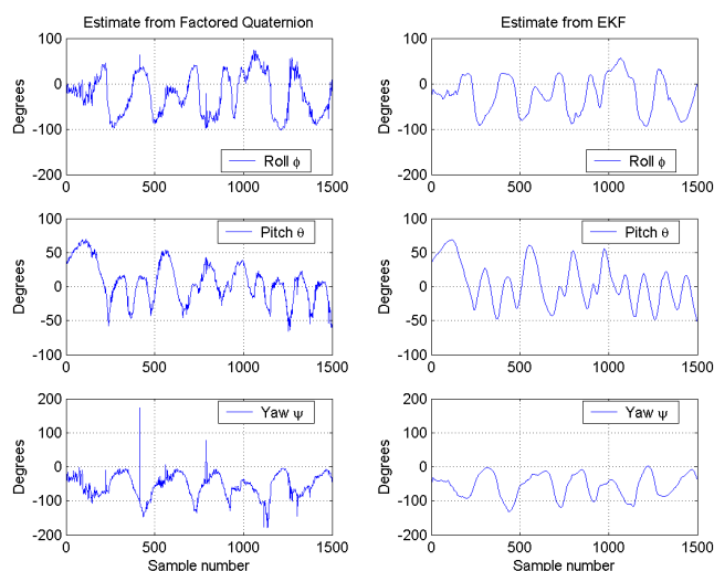
Figure 6. Quaternion estimates produced by the Factored Quaternion Algorithm (left) and Kalman filter (right) with random arm movements.
