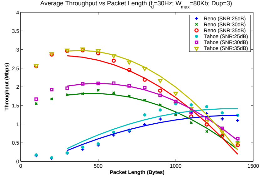
Figure 4.9: Average throughput vs packet length ( f_d=30\text{Hz} ; W_{max}=80\text{Kb} ; Dup=3)
