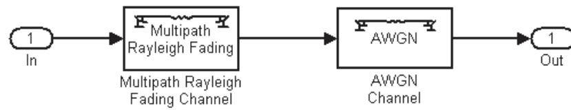
Figure 2.5: Channel blocks for the effect of Doppler spread
