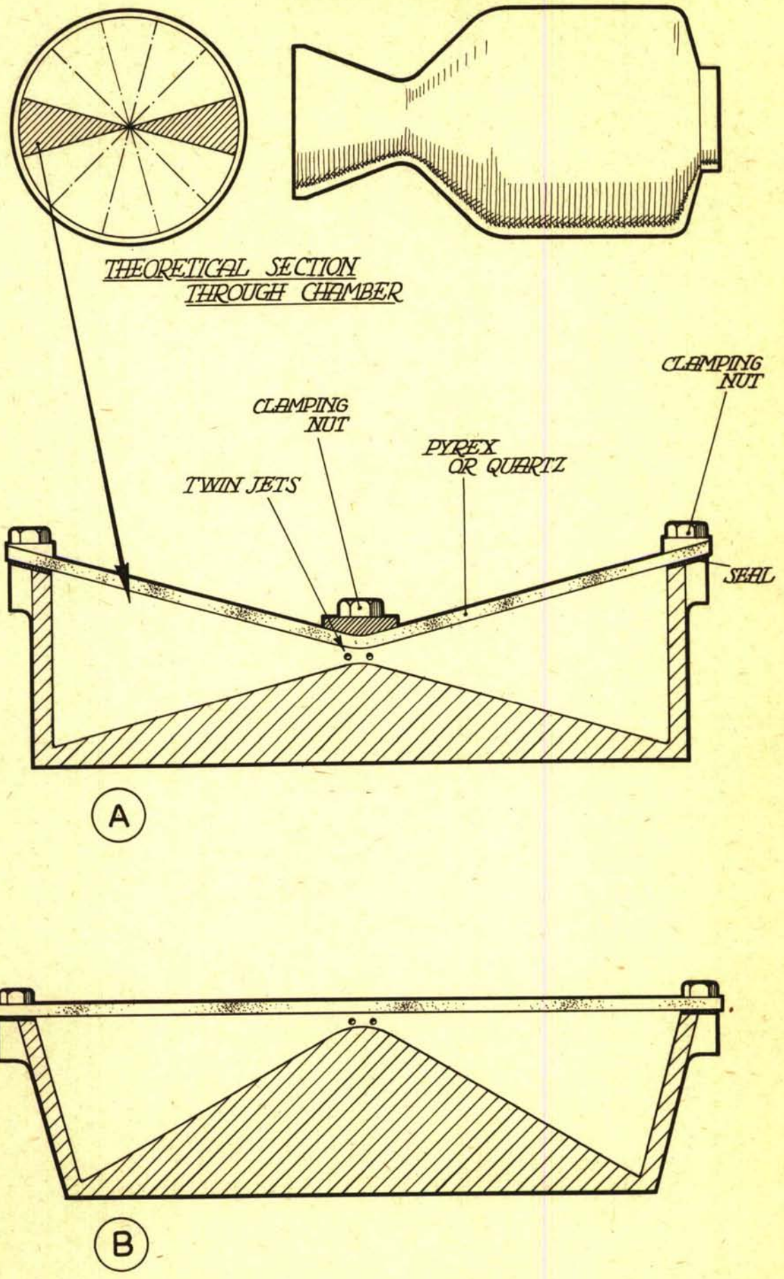
FIG. 1. QUASI THREE DIMENSIONAL MODELS FOR STUDY OF FLOW IN COMBUSTION CHAMBERS
