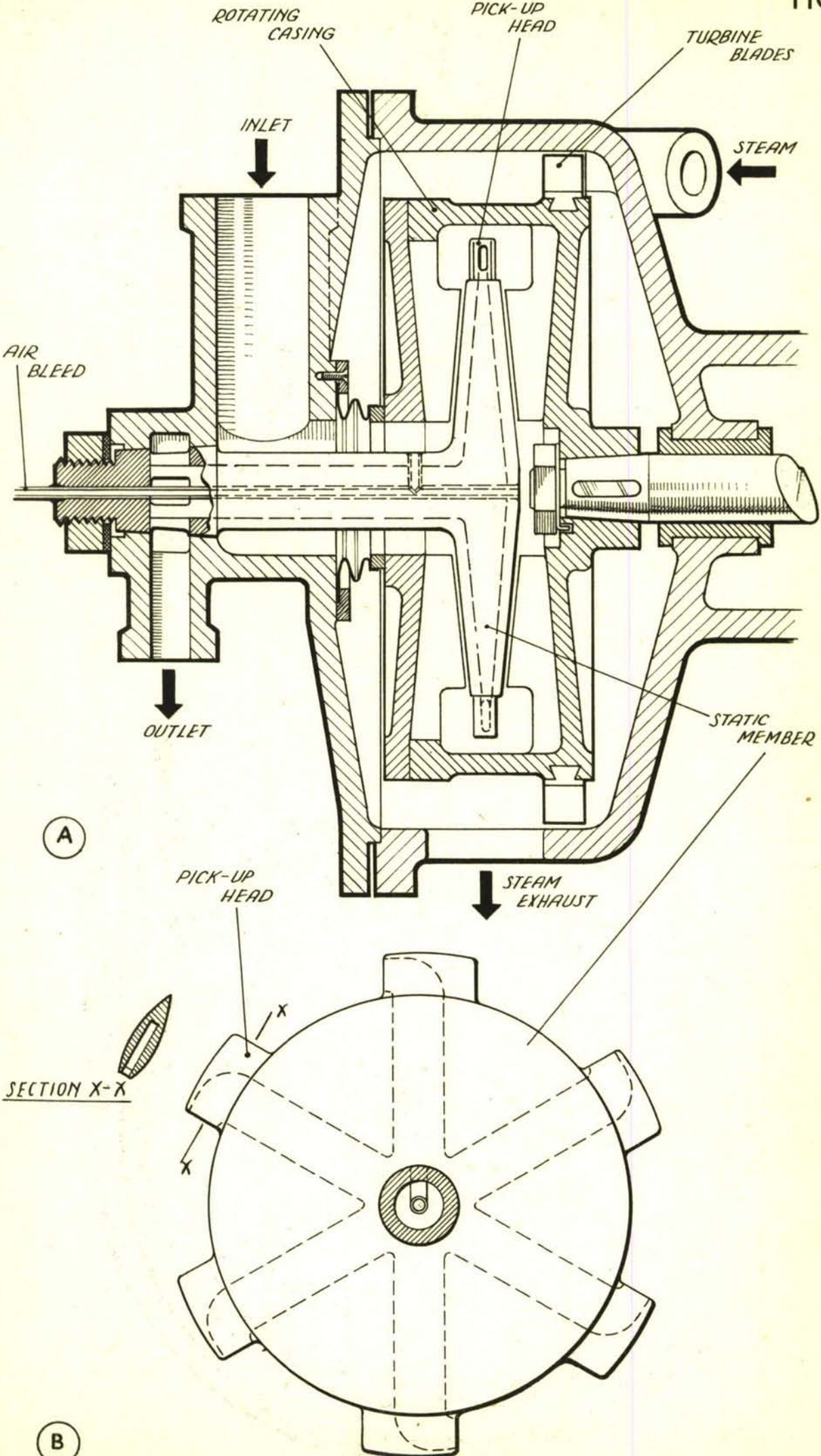
FIG. 11. SCOOP WING PUMP FOR INCREASED FLOW
