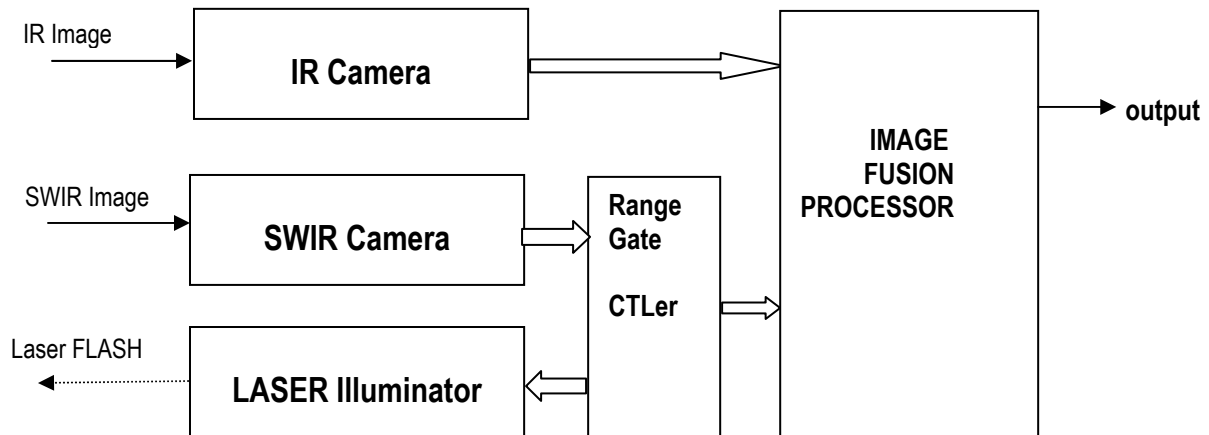
Figure 2: SWIR/IR sensors assembly for image fusion purpose
