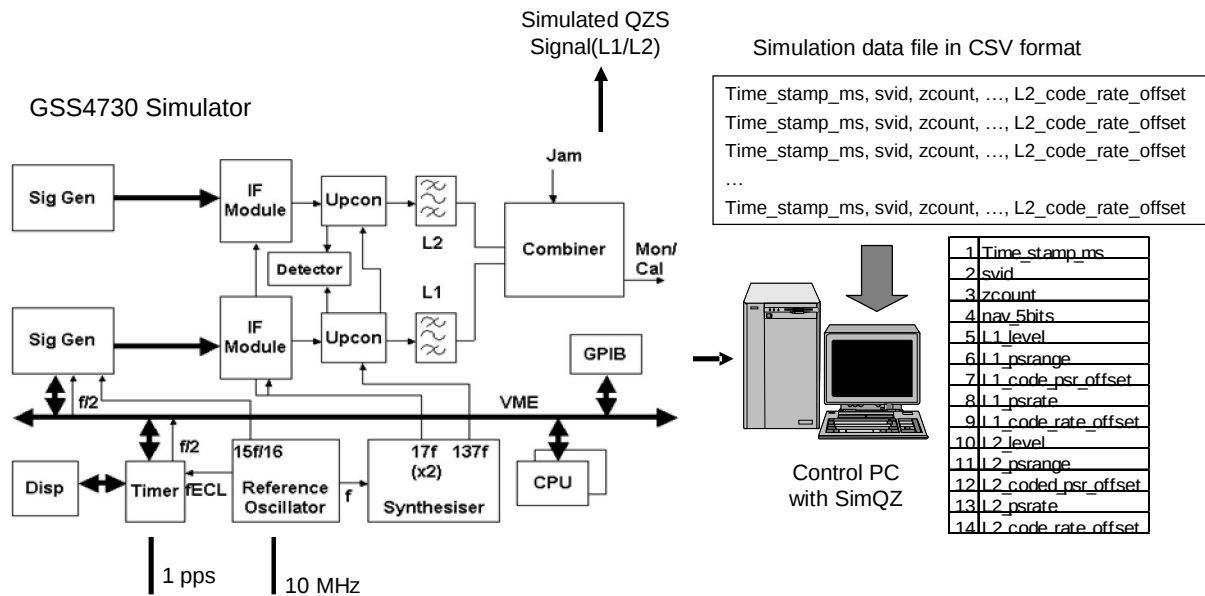
Fig. 7. Block diagram of the QZS signal generator.
