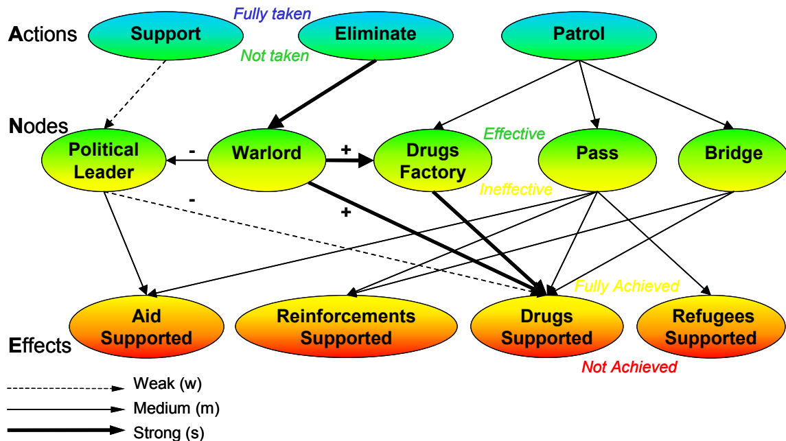
Figure 2: Simple Domain Model
