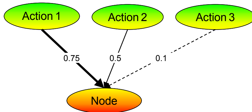
Figure 1: Simplified Influence Weighting
