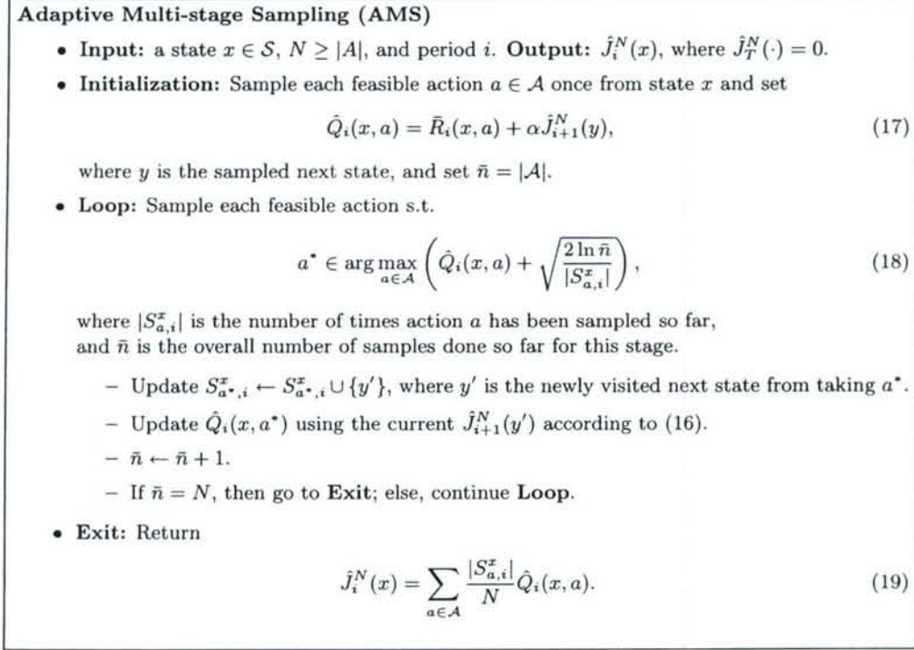
Figure 1: Algorithm incorporating adaptive sampling.
