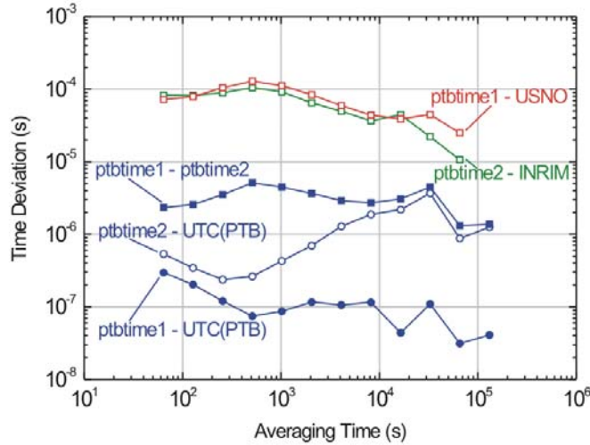
Figure 6. Time deviation (TDEV) plot of the data displayed in Fig. 4. For details, see the text.
