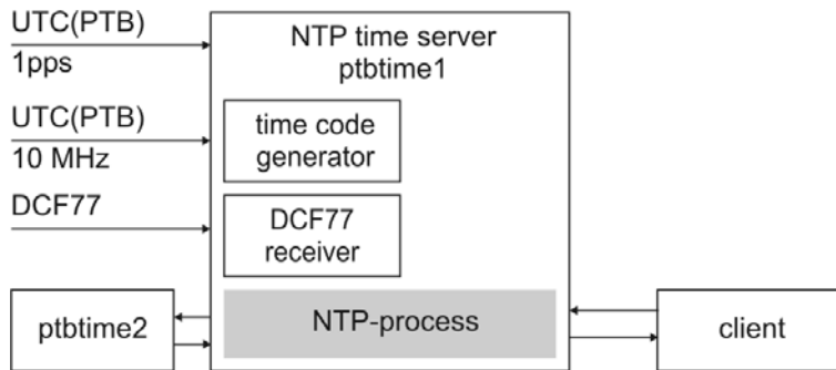
Figure 4. Connection of ptbtime1 to UTC (PTB).
