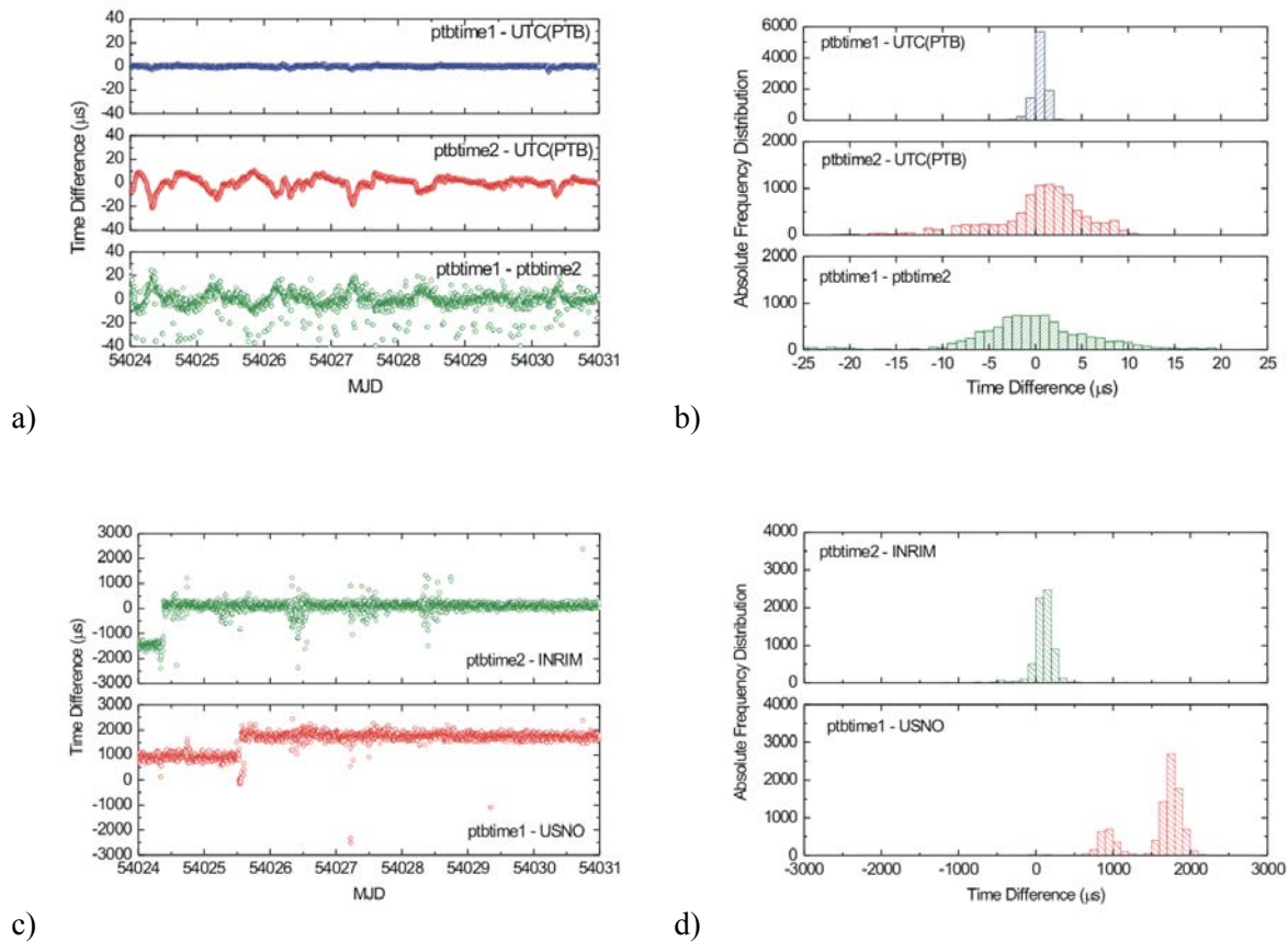
Figure 5. One week (MJD 54025 corresponds to 17 October 2006) of time stamp records with different sources. Time series plot (a) and histogram (b) of comparisons of the internal clock of ptbtime1 and ptbtime2 with the 1pps input UTC (PTB) and ptbtime2 as it is received via the PTB intranet by ptbtime1. Comparison of PTB's NTP server with external servers (c) and (d).
