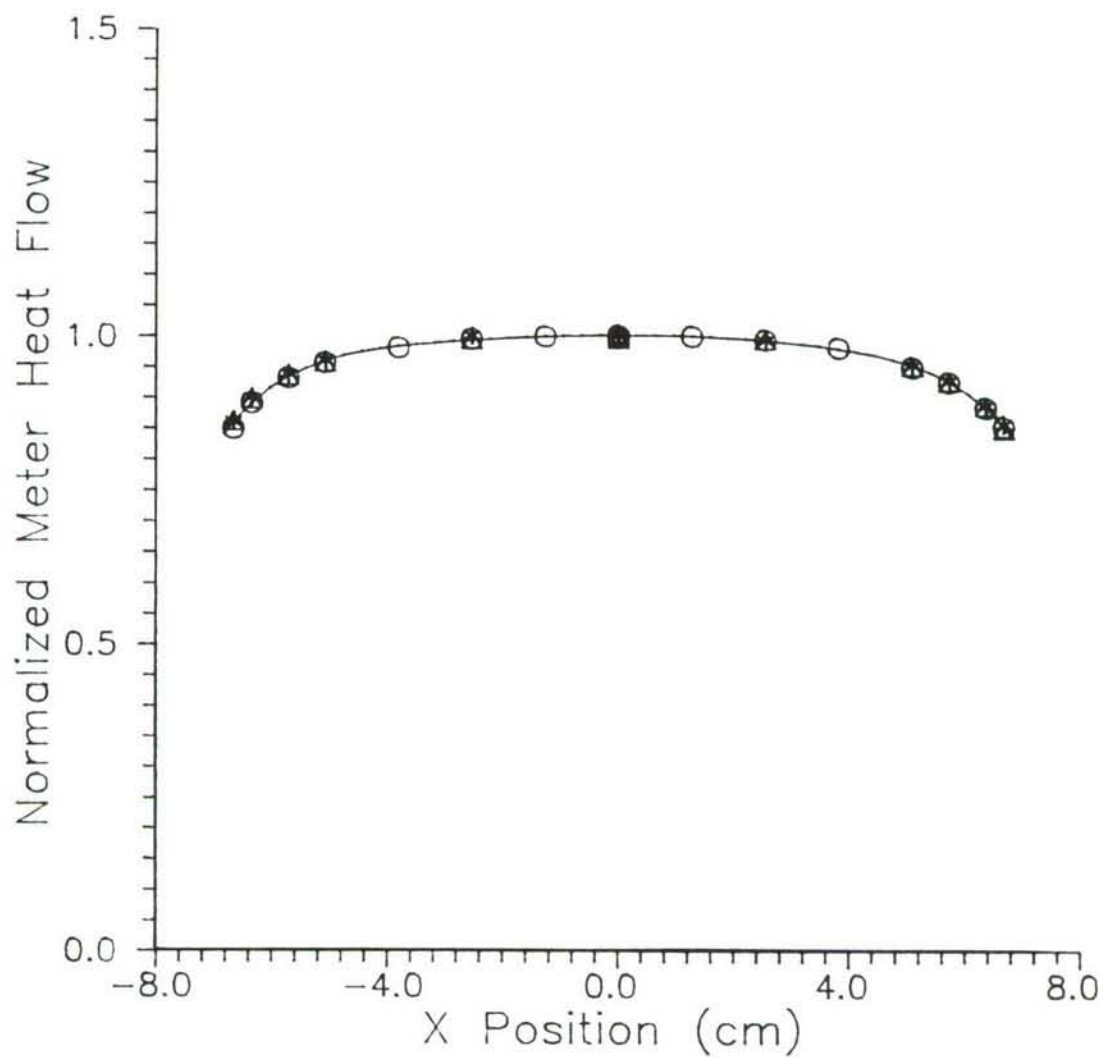
Figure A.5. Traverse of normalized heat flow along x direction at y=0 for heater voltages less than 29%. Shown are data from test 6 (20.4% voltage, "*"), test 9 (20.2% voltage, "o"), and test 10 (24.5% voltage, " \Delta "). The smooth curve is the curve fitted to the normalized heat flow data (j function), which has a standard deviation of 0.3%.
