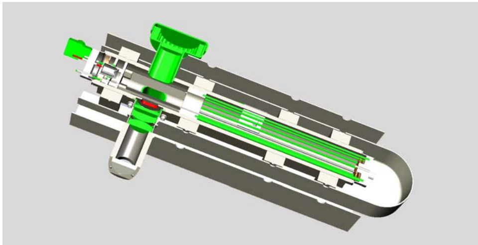
Figure 3. Cutaway design sketch for the 1-liter ion clock physics package layout. The ion tube with two layers of magnetic shielding occupies \sim \frac{1}{4} of the package volume.
