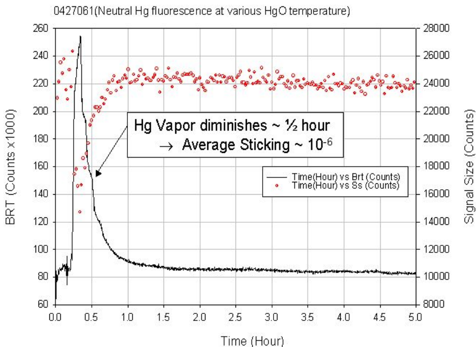
Figure 2. Simultaneous measurements of 194 nm fluorescence from trapped ^{199}\text{Hg}^+ ions (red) and 185 nm neutral ^{199}\text{Hg} vapor (black). HgO oven is brought to \sim 270 C for \sim 1 minute at 0.25 hour. During the \sim 1/2 hour decay of the neutral vapor, the Hg atoms transit the liter-sized tube \sim 10^6 times, demonstrating that the average sticking coefficient for Hg on the internal surfaces is \sim 10^{-6} .
