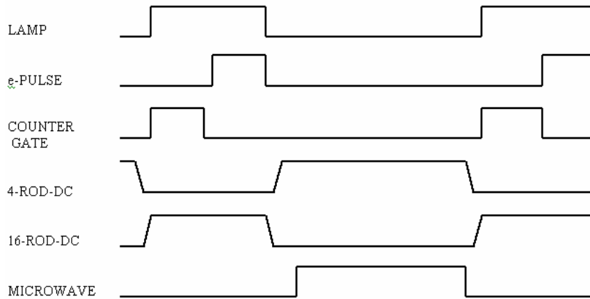
Figure 5. The processor-controlled sequence of operations used to measure local oscillator (LO) frequency.
