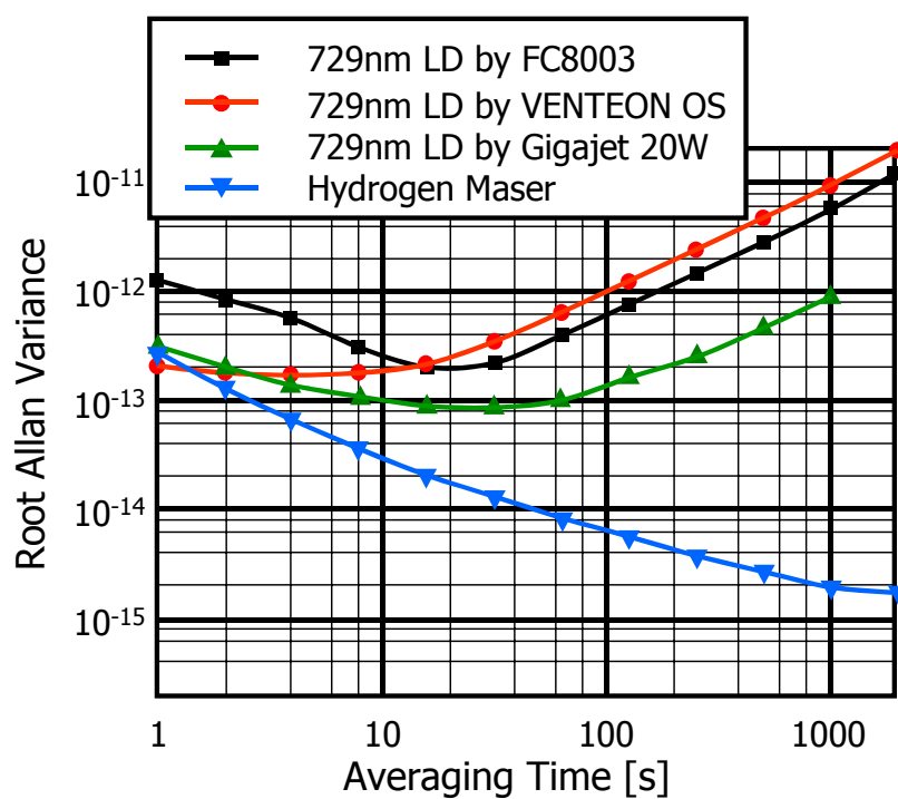
Figure 11. Frequency stability of the clock 729-nm laser measured by three optical frequency combs individually. A hydrogen maser is used as the frequency reference for the frequency combs.
