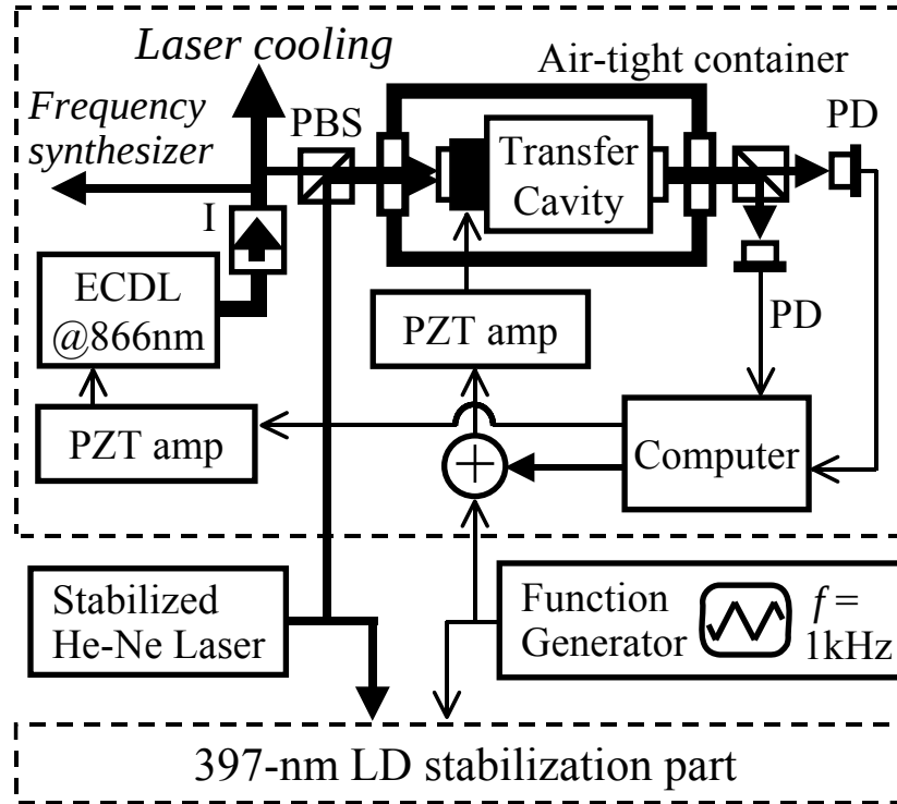
Figure 2. Light source system for laser cooling of ^{40}\text{Ca}^+ ions. ECDL: extended cavity diode laser; I: isolator; PD: photodiode; PBS: polarized-beam splitter; PZT: piezo-transducer.
