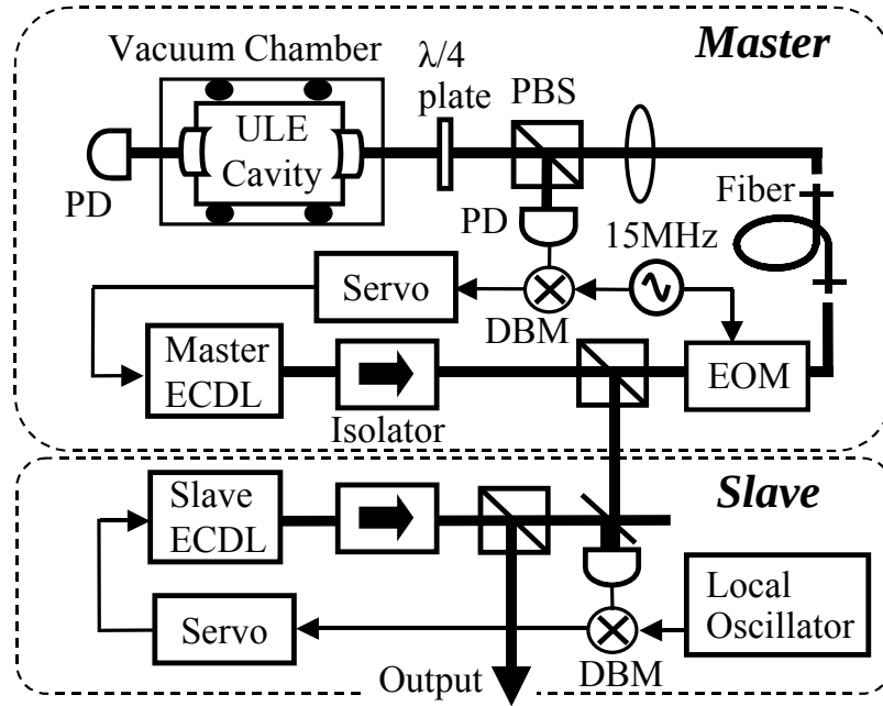
Figure 4. Light source for the quadrupole transition measurement. ULE cavity: ultra-low expansion optical cavity; DBM: double balanced mixer; EOM: electro-optic modulator.
