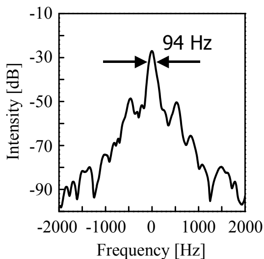
Figure 5. Spectrum of the beatnote between two laser beams stabilized to separate ULE resonant cavities. The linewidth of 66 Hz of each the clock laser is estimated from the linewidth at the -3 dB intensities from the maximum.
