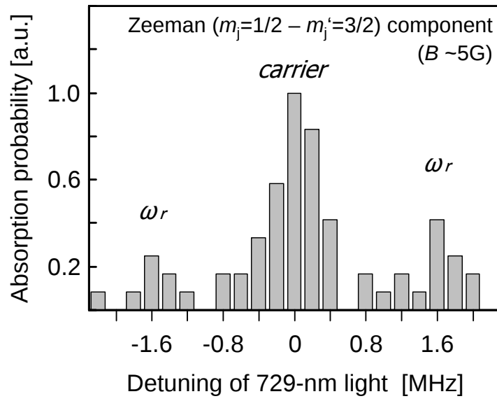
Figure 9. The ^2S_{1/2} - ^2D_{5/2} electric quadrupole transition. This is measured in an external magnetic field of \sim 5 G, and one Zeeman component is shown as a function of the 729-nm frequency detuning.
