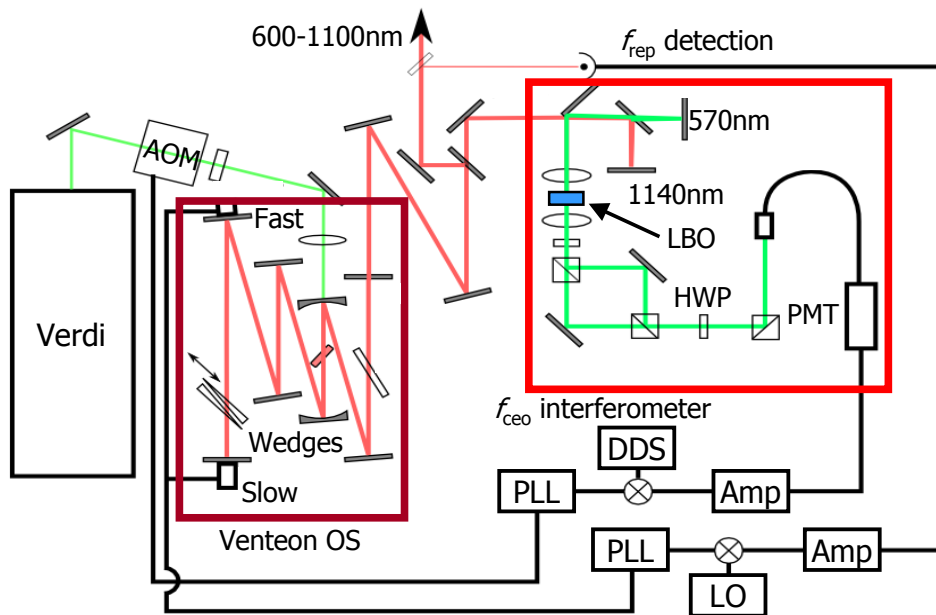
Figure 10. Experimental setup of the optical frequency comb using a VENTTEON OS.
