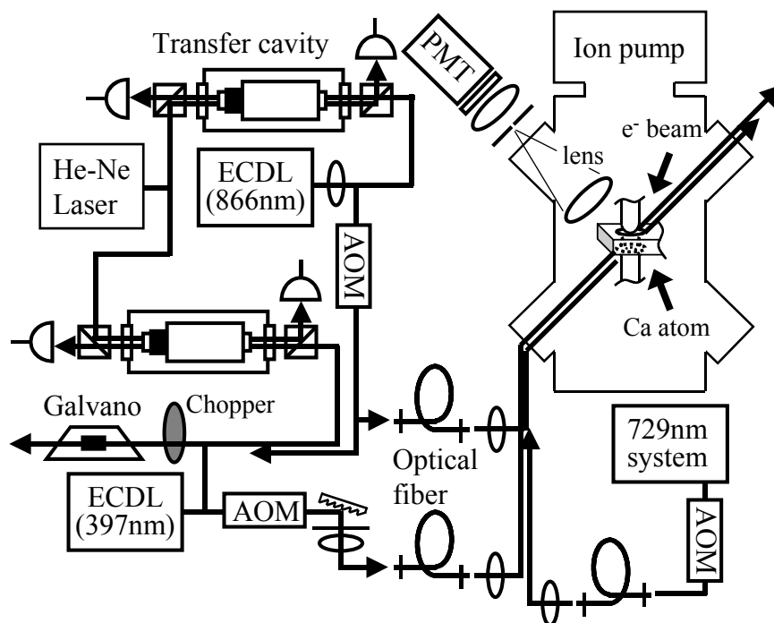
Figure 6. Experimental setup for single ^{40}\text{Ca}^+ ions. AOM: acousto-optic modulator; PMT: photo-multiplier tube; Galvano: Galvano tube.
