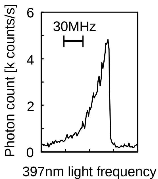
Figure 7. Spectrum of a laser-cooled single ^{40}\text{Ca}^+ ion.
