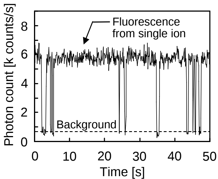
Figure 8. Quantum jumps of a single ^{40}\text{Ca}^+ ion.
