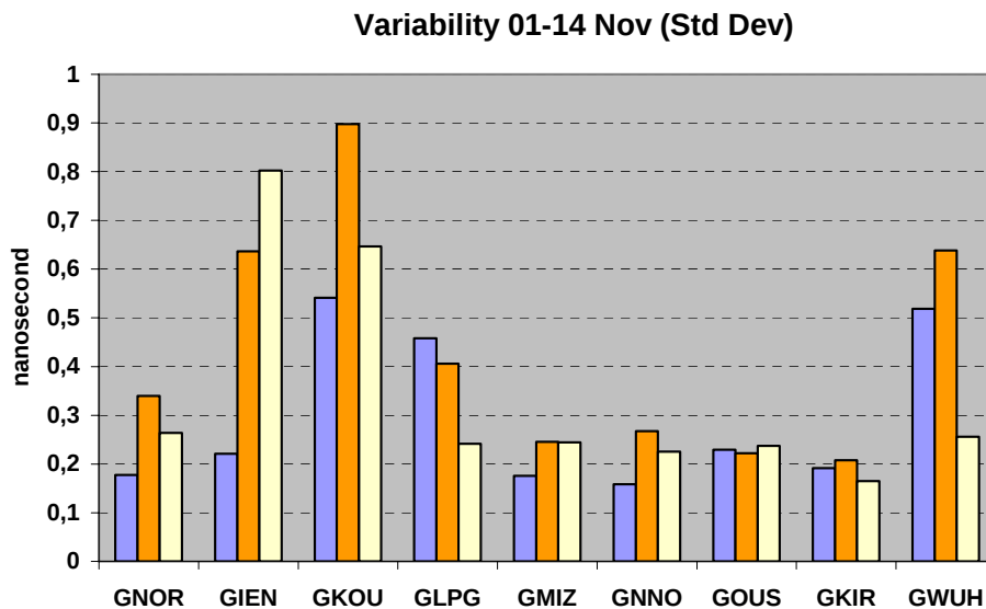
Figure 10. Station IFBs and inter-system biases (variability).
