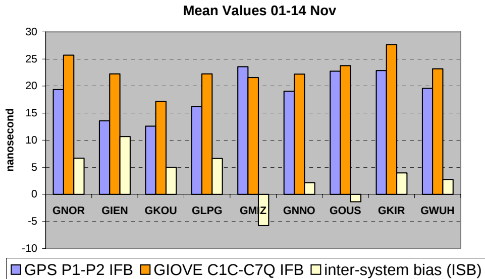
Figure 9. Station IFBs and inter-system biases (mean values).
