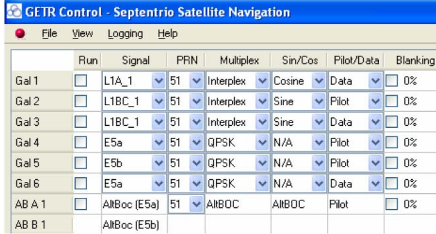
Figure 4. The GETR receiver configuration.
