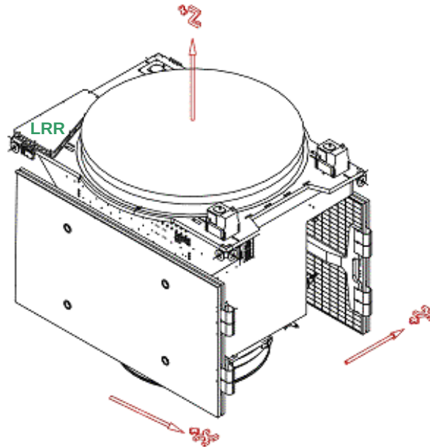
Figure 1. GIOVE-A in stowed configuration.
