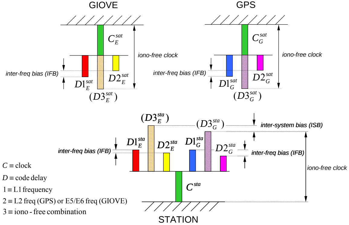
Figure 5. Timing biases in GSTB-V2.
