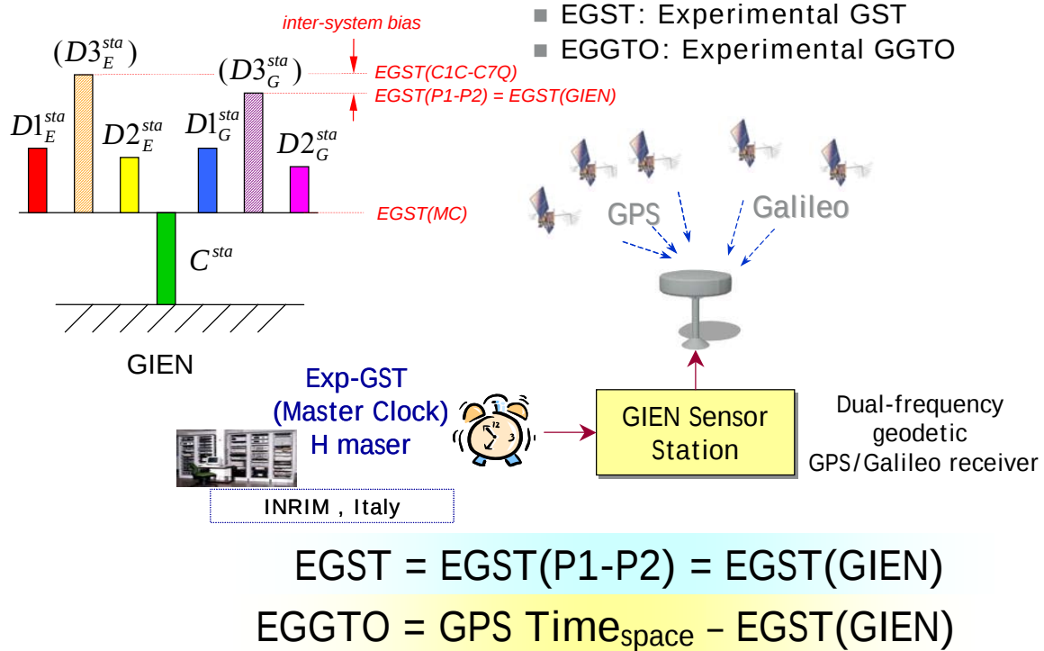
Figure 7. The EGST and EGGTO concepts in GSTB-V2.
