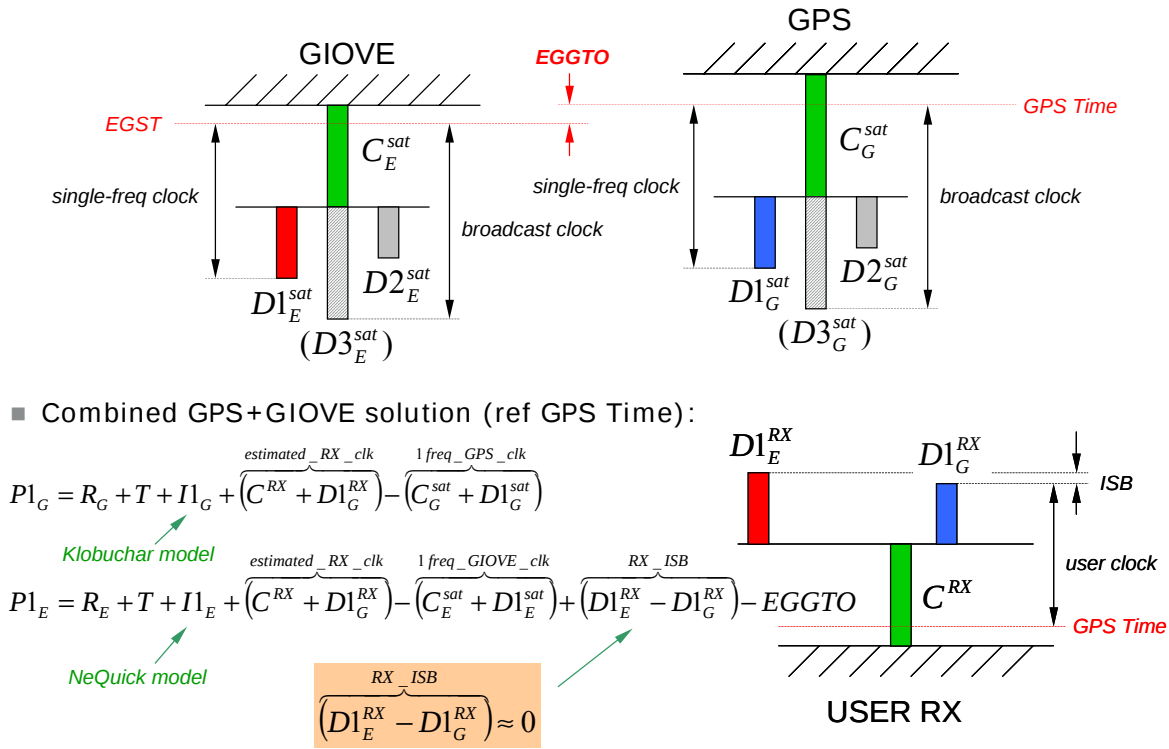
Figure 11. User solution for a single-frequency receiver.
