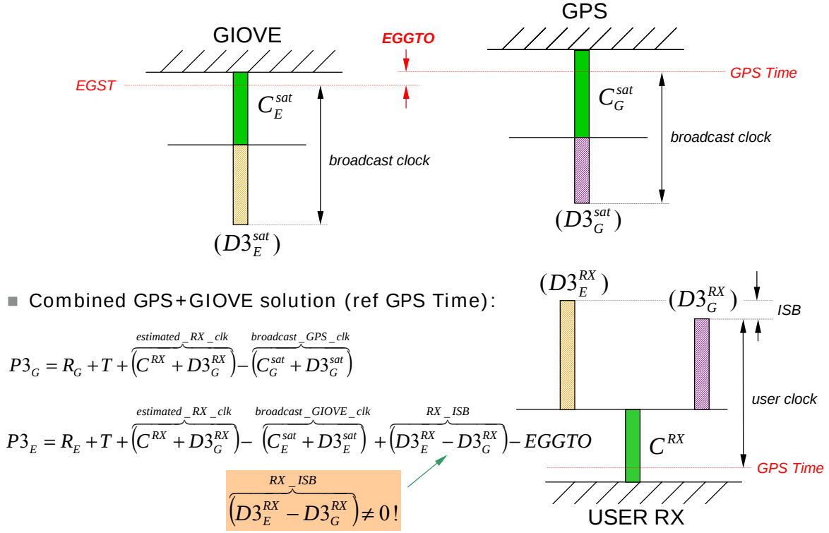
Figure 12. User solution for a dual-frequency receiver.
