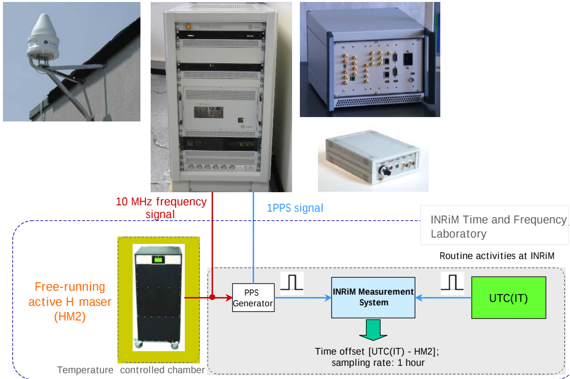
Figure 2. Elements of the Galileo Experimental Sensor Station (GESS).
