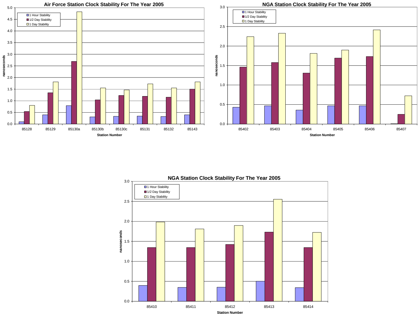
Figure 5. Station clock (frequency to time) stability of the AF and NGA monitor stations for the year 2005. The top chart shows the stability of the AF monitor computed by the NGA Kalman filter process. This chart shows the improvement at the Diego Garcia (85130) station with the upgrade to the new 5071A CFS. The second chart shows the NGA monitor stations that were included in the Aii process in the early fall of 2005. Stations at Colorado Springs (85128) and at the USNO (85407) statistics are much better due to being hydrogen masers. The 1/2-day stability statistics are used by NGA for quality control and are approximates. The bottom chart shows the stations to be included in future Aii plans. The station 85413 (South Korea) has the highest values due to the numerous maintenance problems. Stations 85411 (New Zealand) and 85412 (South Africa) were recently added to the Aii process. Note text for the explanation.
