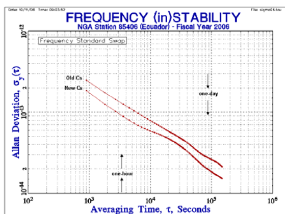
Figure 6. The AF station at Kwajalein changed frequency standard at the beginning of the year 2006. The stability plot is very similar to the stability in Figure 2. The NGA station at Ecuador upgraded the cesium beam tube of an older 5071A frequency standard in mid-June 2006. Note the improved frequency and stability of the old versus the new cesium standards.
