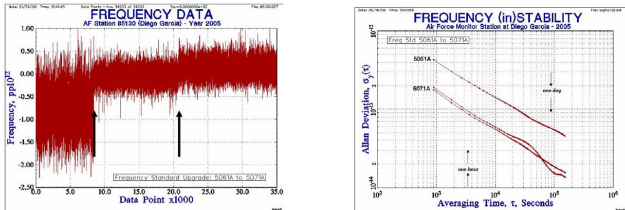
Figure 3. The AF station at Diego Garcia was upgraded from a CFS 5061A to a CFS 5071A about one quarter the way through 2005. The first arrow (left), on the frequency data plot, shows the large improvement in the frequency data noise. The second arrow (right), on the frequency data plot shows a small jump in the frequency. This corresponds to a start-up of the second CFS 5071A. The stability plot shows the improvement.
