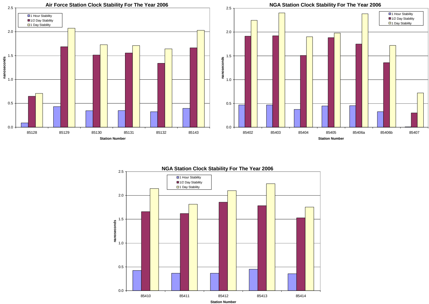
Figure 7. Station clock (frequency to time) stability of the AF and NGA monitor stations for the fiscal year 2006. The top chart shows the stability of the AF monitor computed by the NGA Kalman filter process. The second chart shows the NGA monitor stations that were included in the Aii process in the early fall of 2005. This chart shows the improvement at the Ecuador (85406) station with replacement of the CFS. Stations at Colorado Springs (85128) and at the USNO (85407) have statistics that are much better due to being hydrogen masers. The 1/2-day stability statistics are used by NGA for quality control and are approximates. The bottom chart shows the stations to be included in future Aii plans. The station 85413 (South Korea) has the highest values due to the numerous maintenance problems. Stations 85411 (New Zealand) and 85412 (South Africa) were recently added to the Aii process. Note text for the explanation.
