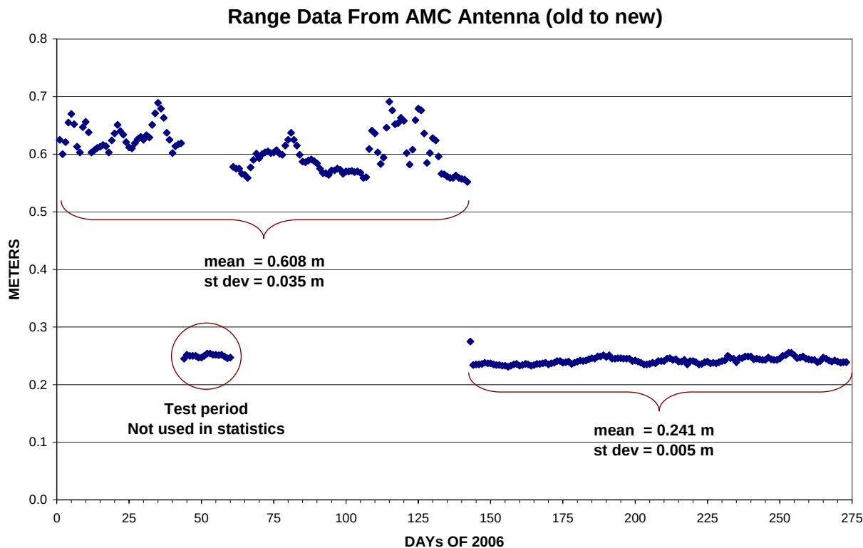
Figure 8. Range data received from the antennas at Schriever Air Force Base (AMC1). For days 001 to 142, note the higher mean value. This was due to multi-path problems (?) due to a large dome over the antenna. The new antenna, which replaced the old, does not have this problem. Note the improvement in the mean from day 143 onward. The test period from days 44 to 60 shows a similar improvement in the data. Also, note the lower standard deviation from the new antenna compared with the old antenna. There is currently no dome over the new antenna.
