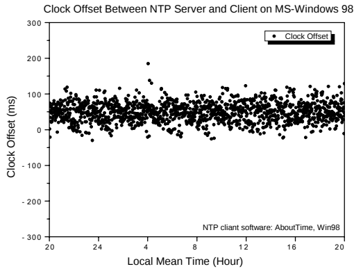
Figure 3. Clock offset of the NTP time synchronization between the GPS-based NTP time server and the local PC clock with an MS-Windows 98 OS.
