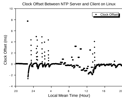
Figure 6. Clock offset of the NTP time synchronization between a GPS-based NTP time server and a local PC clock on Linux OS.
