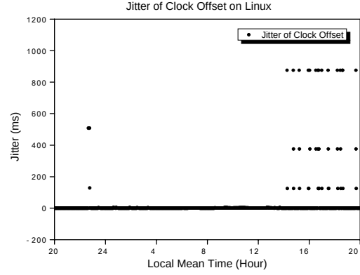
Figure 8. Jitter of clock offset on Linux OS.
