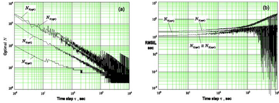
Figure 3: Optimal N_{\text{opt}} vs. \tau for the first clock state (TIE): (a) optimal N and (b) RMSE.
