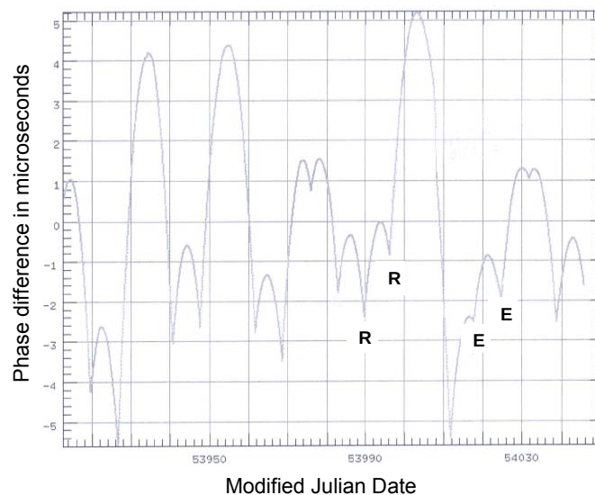
Figure 5. Phase of syntonized micro-stepper to H maser reference.
