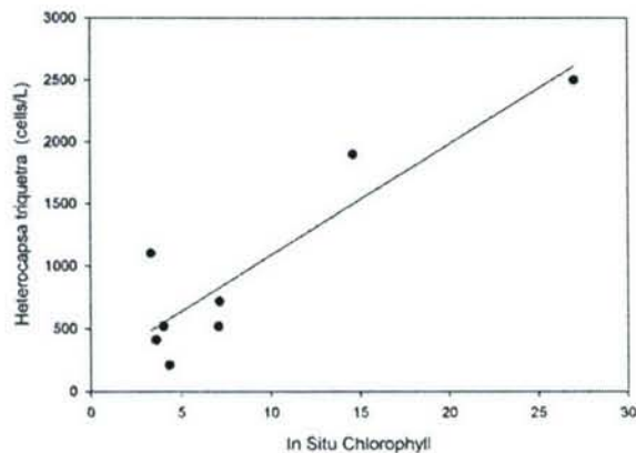
Figure 3. Heterocapsa triquetra cell count vs. Chla ( r^2= 0.826 ).
