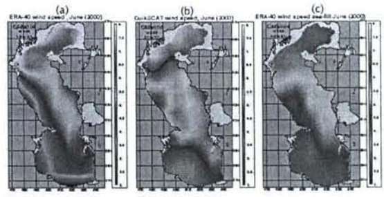
Fig. 2. Spatial variations of wind speed from ECMWF, QSCAT and sea-fill field.
