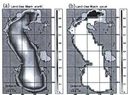
Fig. 1. The land sea mask from a satellite-based product (QSCAT, right), and ECMWF interpolated to the 1/25° grid (left)
