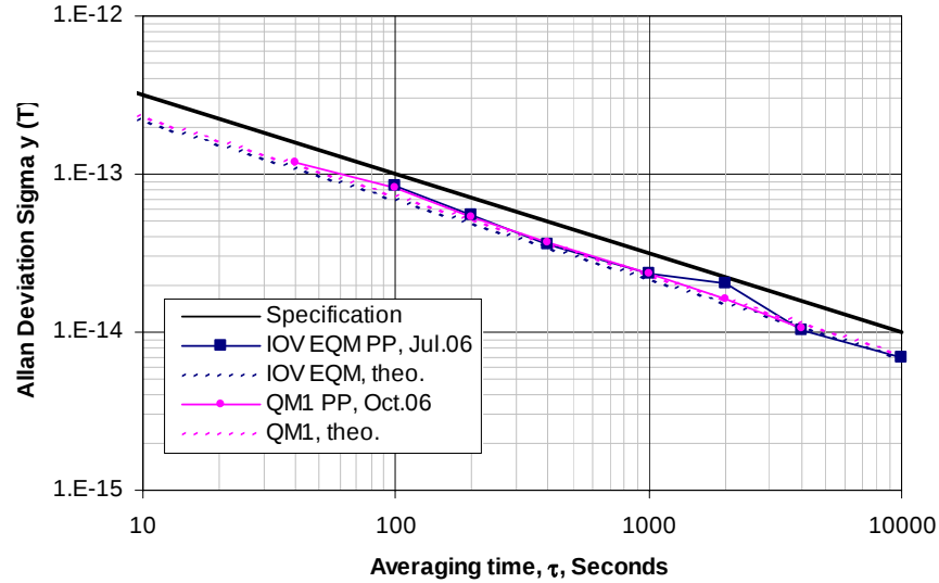
Figure 12. Measured and theoretical frequency stabilities of Physics Packages for the IOV EQM and QM1.
