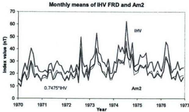
Figure 2. Comparison of monthly means of the “raw” IHV index (blue) calculated for the H component at Fredericksburg and the Am2 index (red) for the interval 1970–1976. The year labels on the abscissa mark the beginning of each year. The thin pink curve shows IHV scaled down by 0.7475 for direct comparison with Am2 . Note that Am2 is the average am index for two 3-hour intervals.
