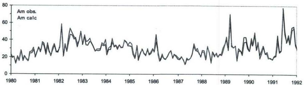
Figure 9. (top) Bartels rotation averages of proxy values of Am calculated using equation (4) (blue curve) and observed (red curve). Both data sets have been freed from the effect of the dipole tilt (section 3.2). Also shown are (bottom) the entire data sets overlain by their 13-rotation running means.
